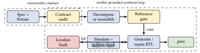
Figure 2: C4tl pipeline. The method first establishes an executable contract, then validates a reference decomposition before entering a golden-feedback loop. On failure, swap-based localization chooses one culprit module for targeted repair.
