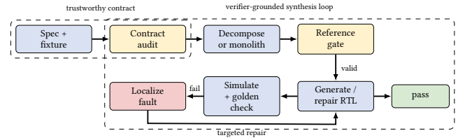
Figure 2: C4tl pipeline. The method first establishes an executable contract, then validates a reference decomposition before entering a golden-feedback loop. On failure, swap-based localization chooses one culprit module for targeted repair.
