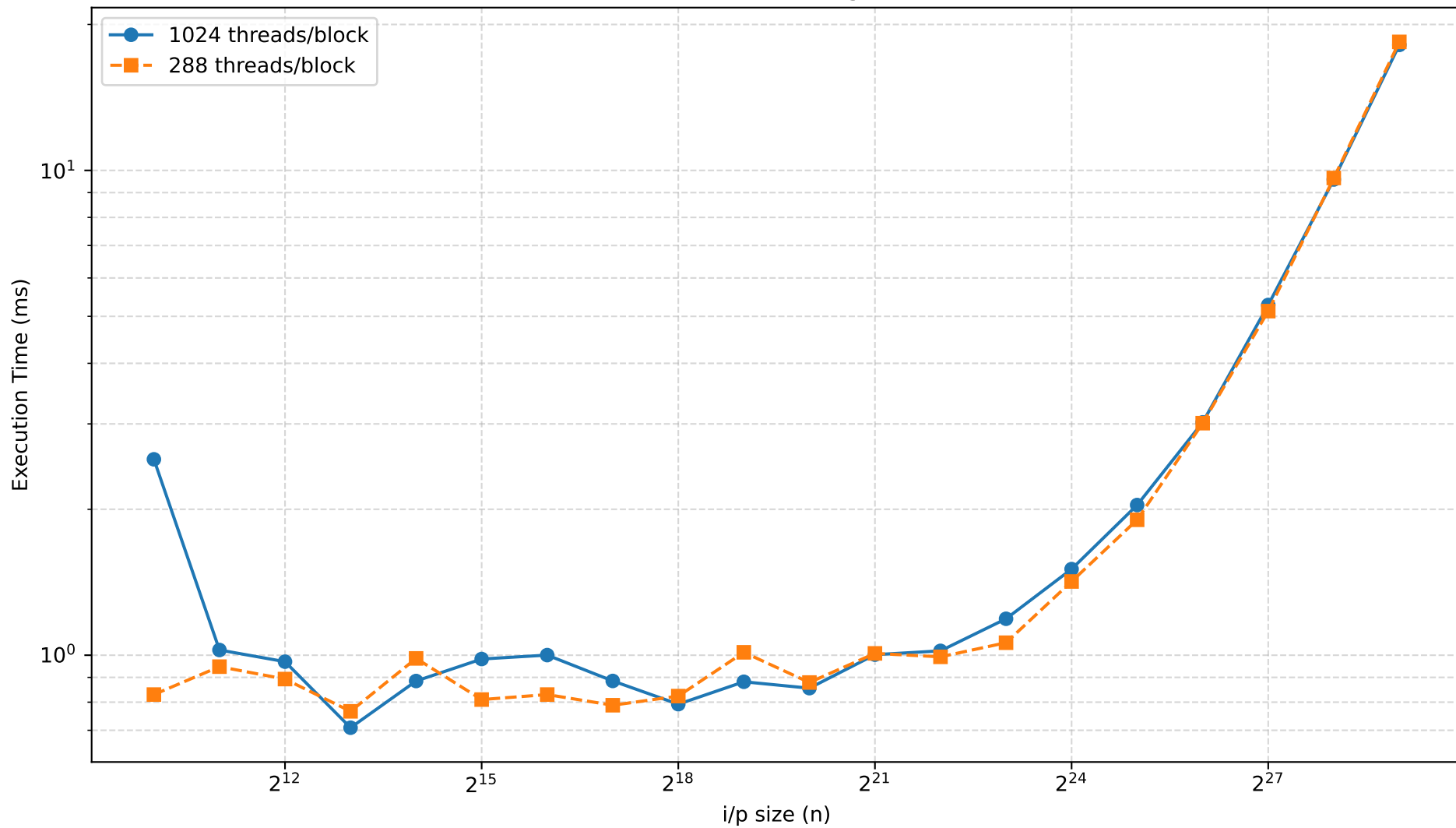
CUDA Scaling
