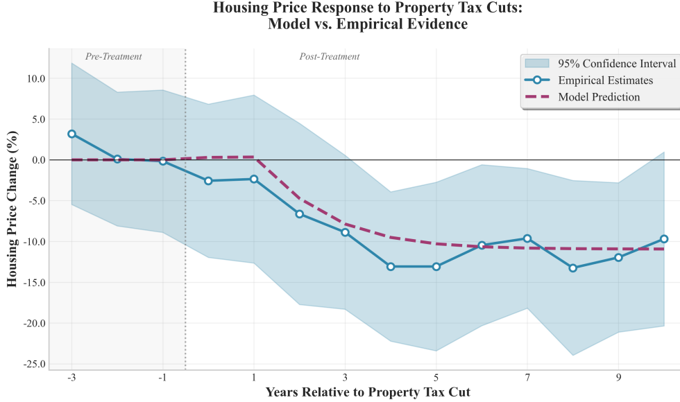
Figure 17: Model vs Empirical Estimates of House Prices Following the Tax Cut.
