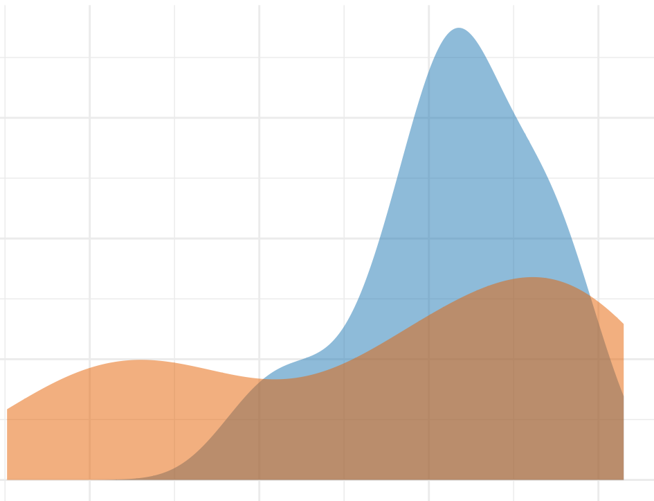
Distribution of Spearman's r by Cluster
