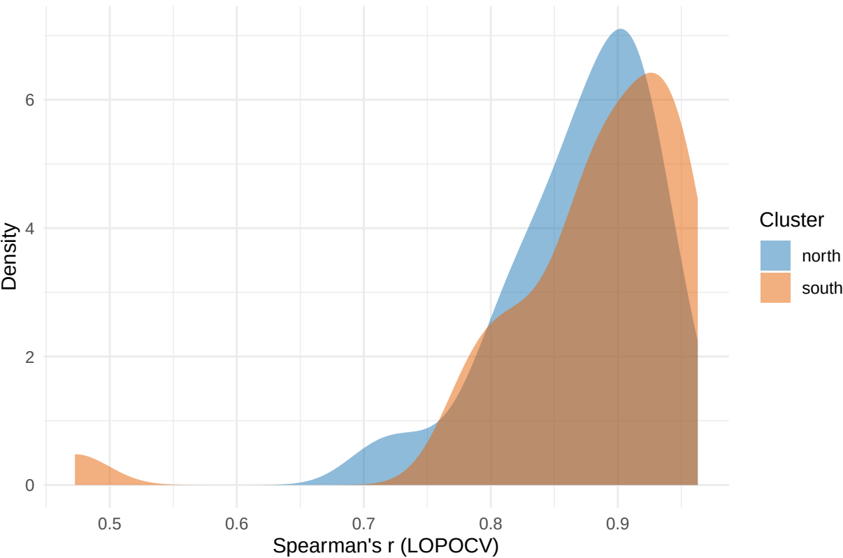
Distribution of Spearman's r by Cluster
