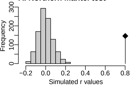
A. Northern Mantel test
