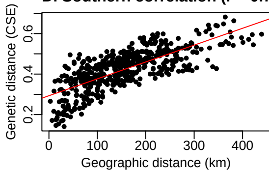
D. Southern correlation ( r = 0.75 )
