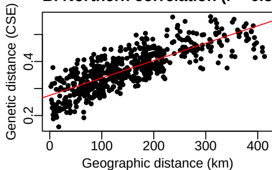
B. Northern correlation ( r = 0.80 )
