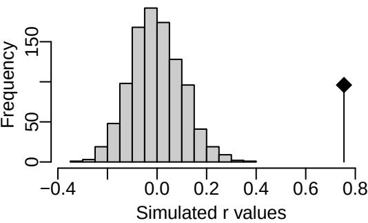
C. Southern Mantel test
