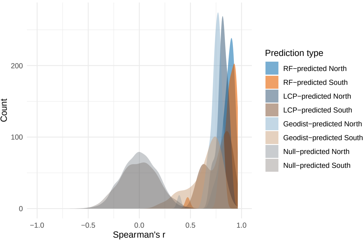
Fold-level LOPOCV Spearman by prediction type and cluster
