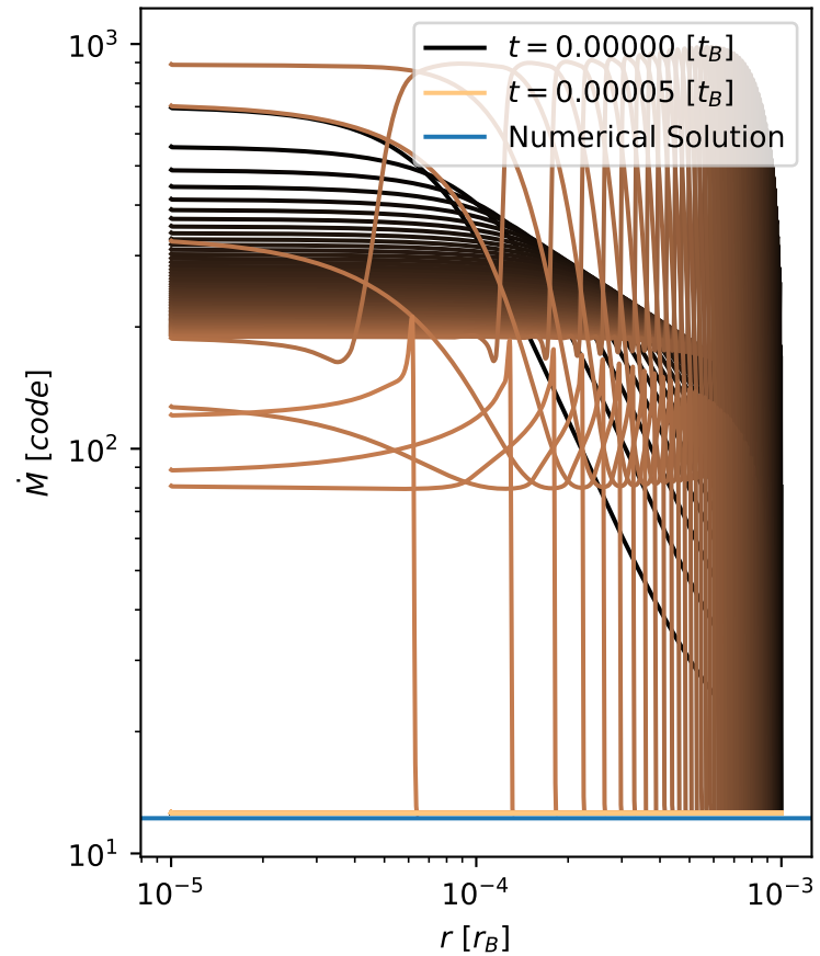
Mass accretion
