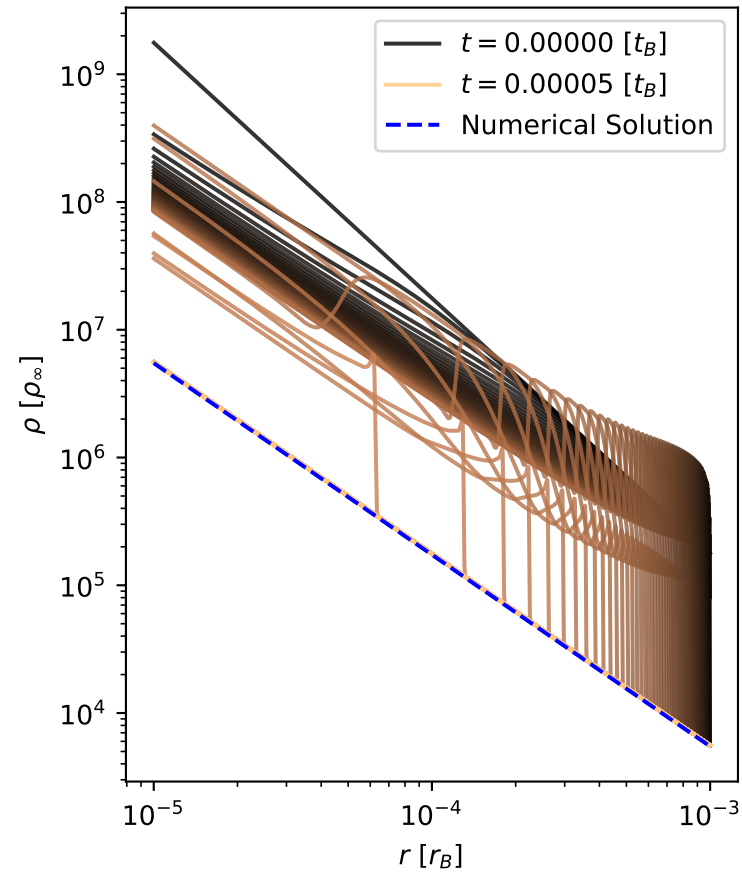
Density evolution
