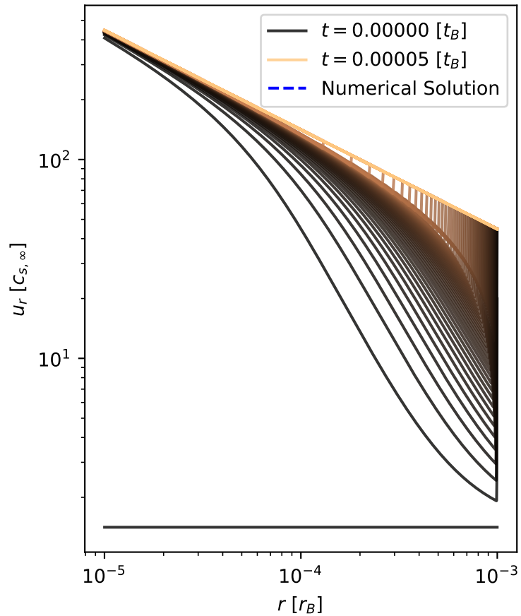
Velocity evolution
