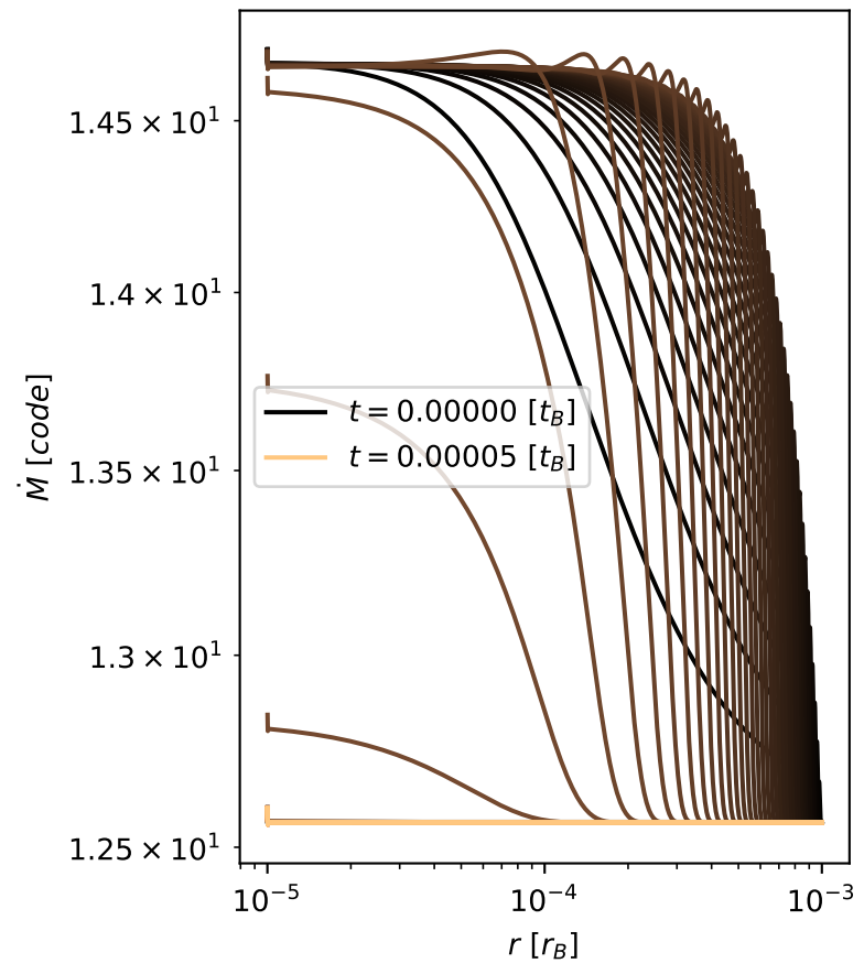
Mass accretion
