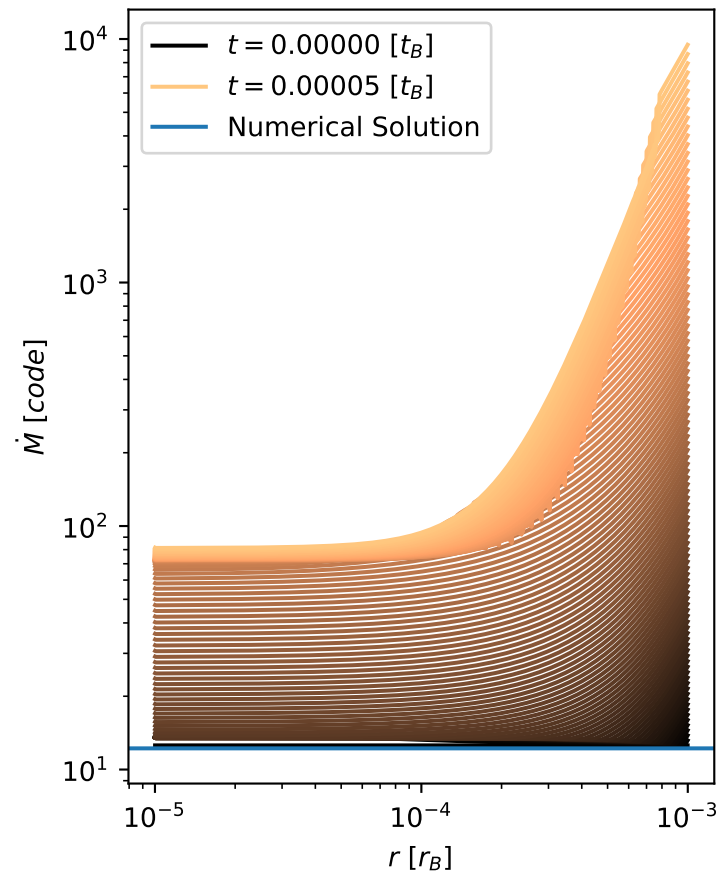
Mass accretion
