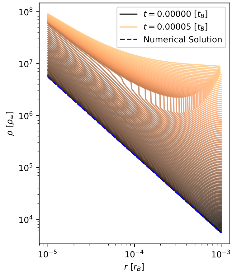
Density evolution
