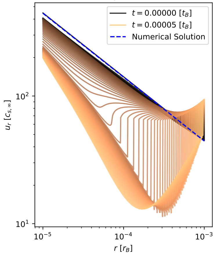
Velocity evolution
