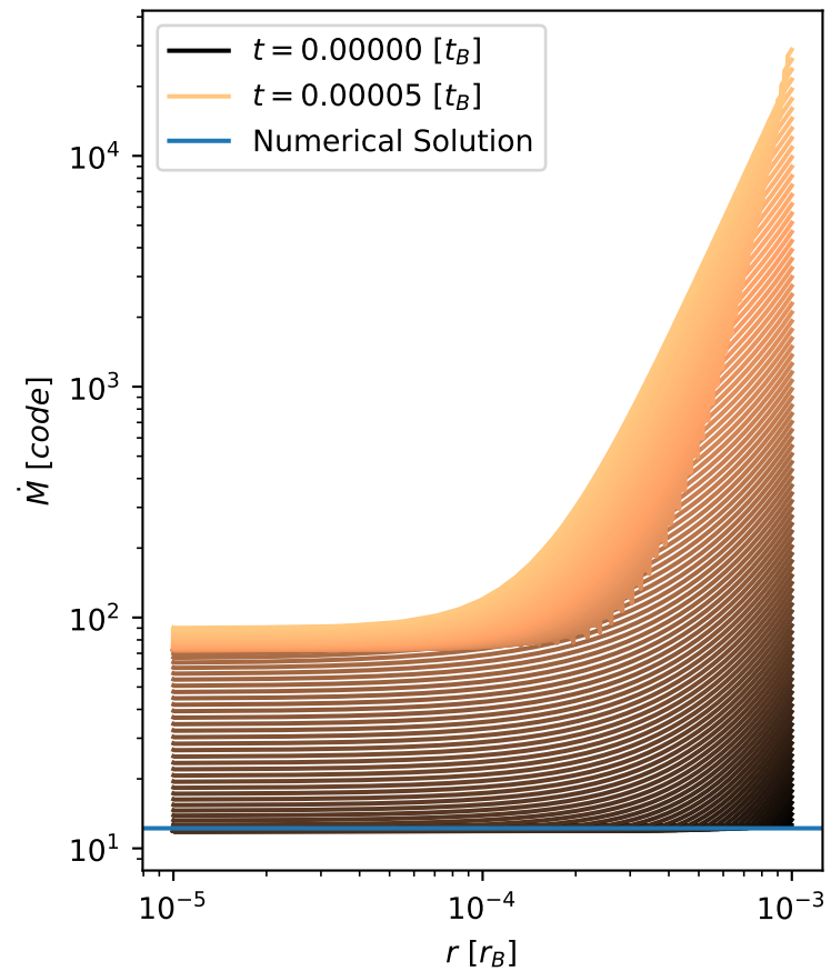
Mass accretion
