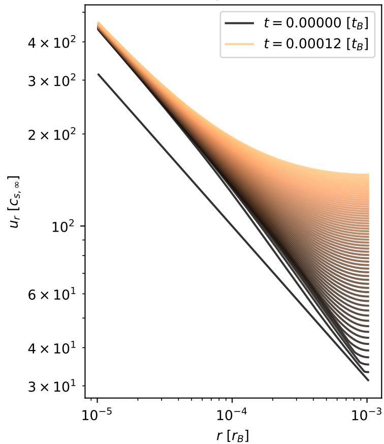
Velocity evolution
