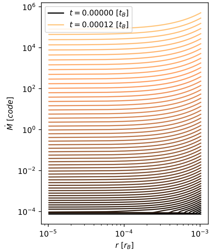
Mass accretion
