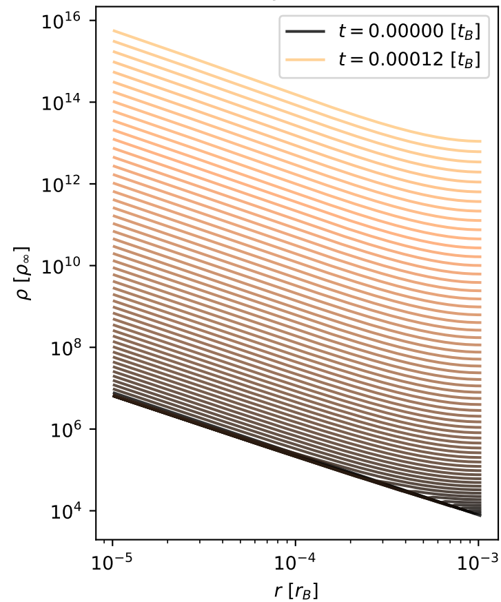
Density evolution
