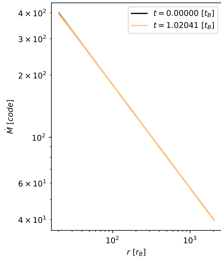
Mass accretion
