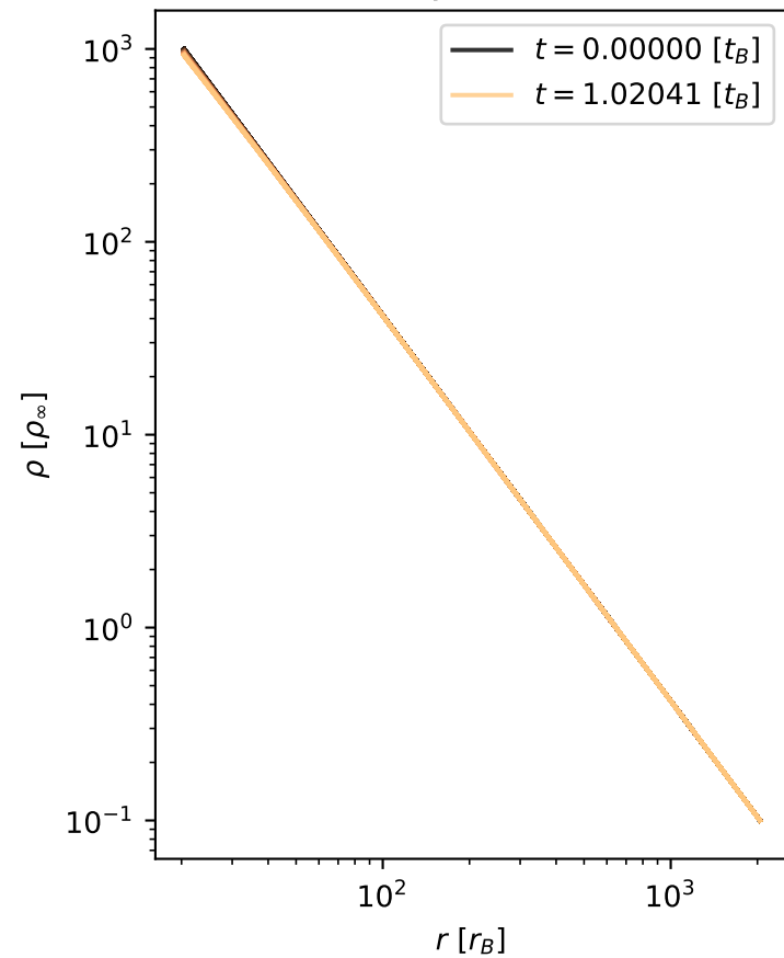
Density evolution
