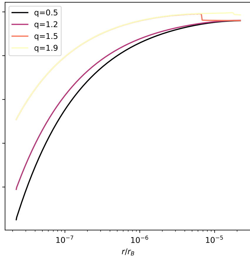
Final velocity profiles
