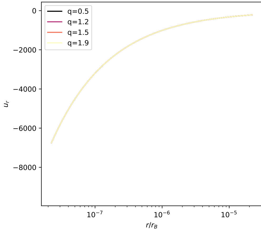
Initial velocity profiles
