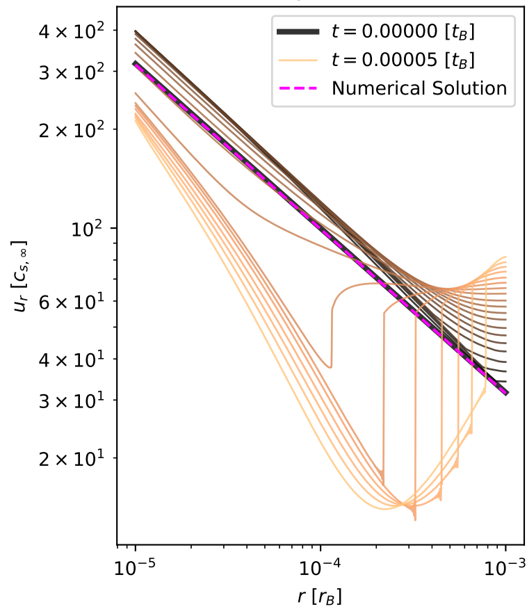
Velocity evolution
