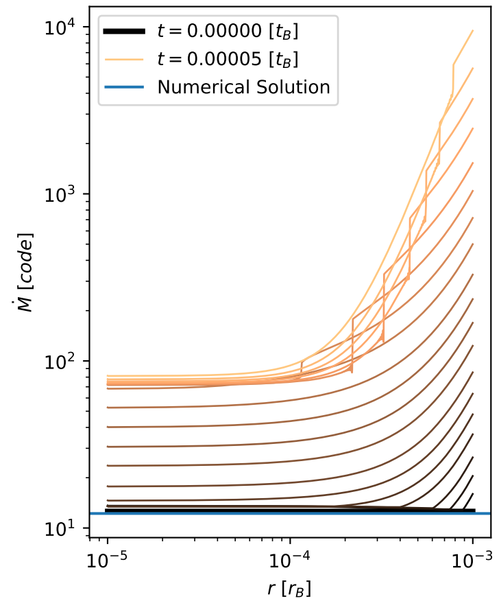
Mass accretion
