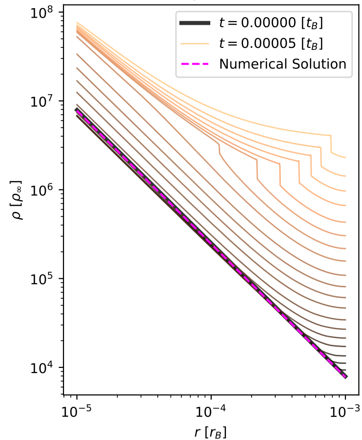
Density evolution
