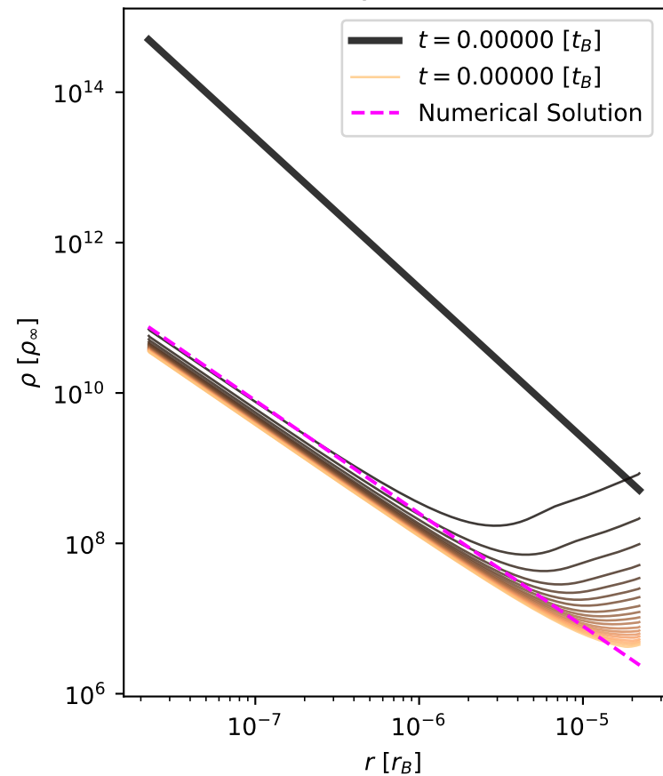
Density evolution
