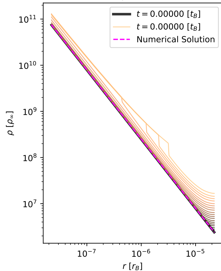
Density evolution
