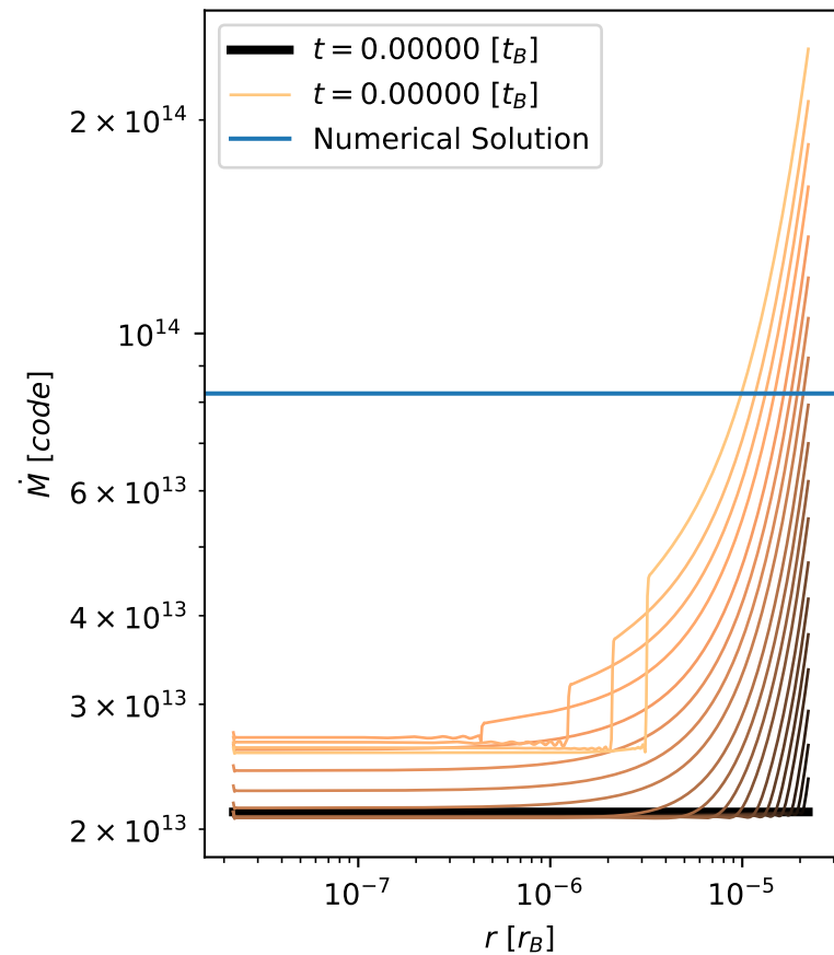
Mass accretion
