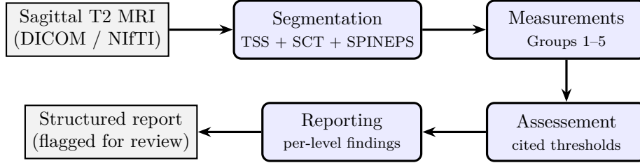
Figure 1: End-to-end pipeline. Segmentation delegates to three engines; measurements are organized into five groups; assesment classifies each measurement against a cited-threshold catalog; reporting emits per-level findings flagged for physician review.
