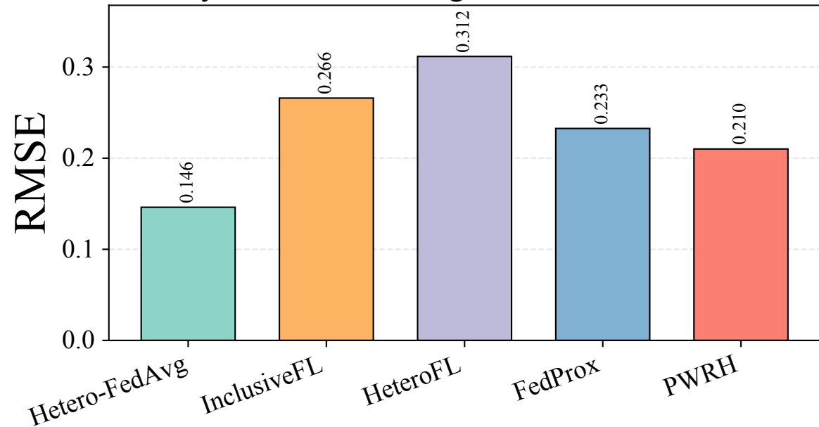
1-Layer Clients: Average Best Validation RMSE
