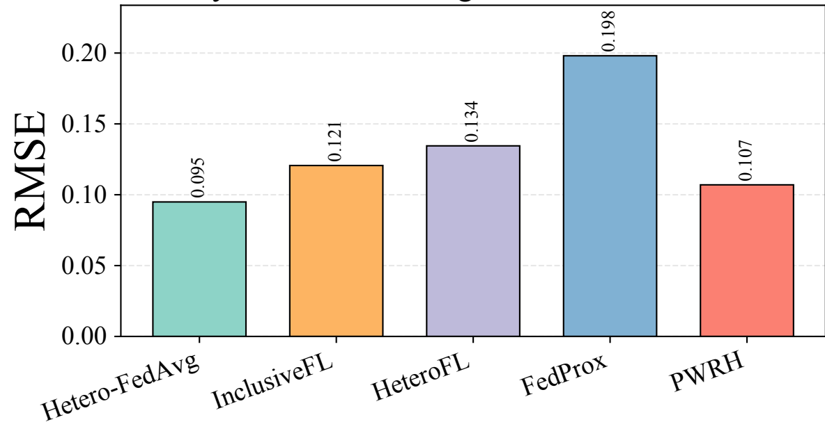
2-Layer Clients: Average Best Validation RMSE
