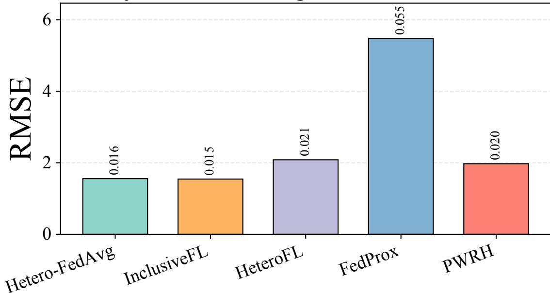
3-Layer Clients: Average Best Validation RMSE
