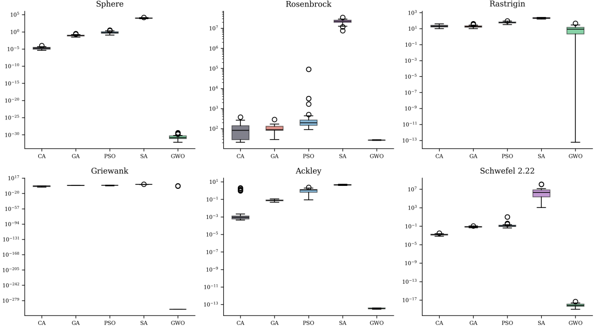
Figure 3: Distribution of final objective values over 30 runs.
