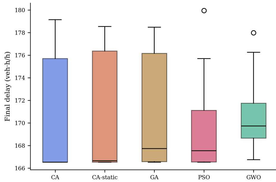
Figure 19: Distribution of final delays over 30 runs.
