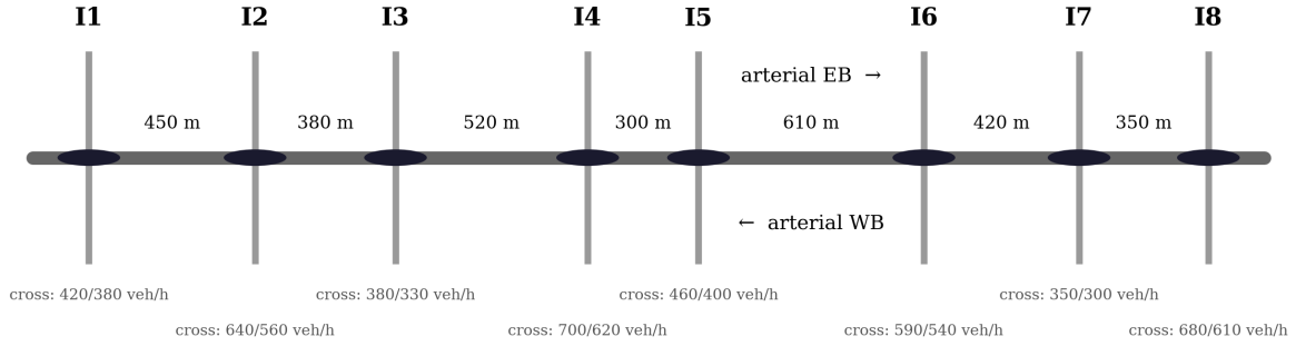
Figure 16: Layout of the eight-intersection arterial test bed.
