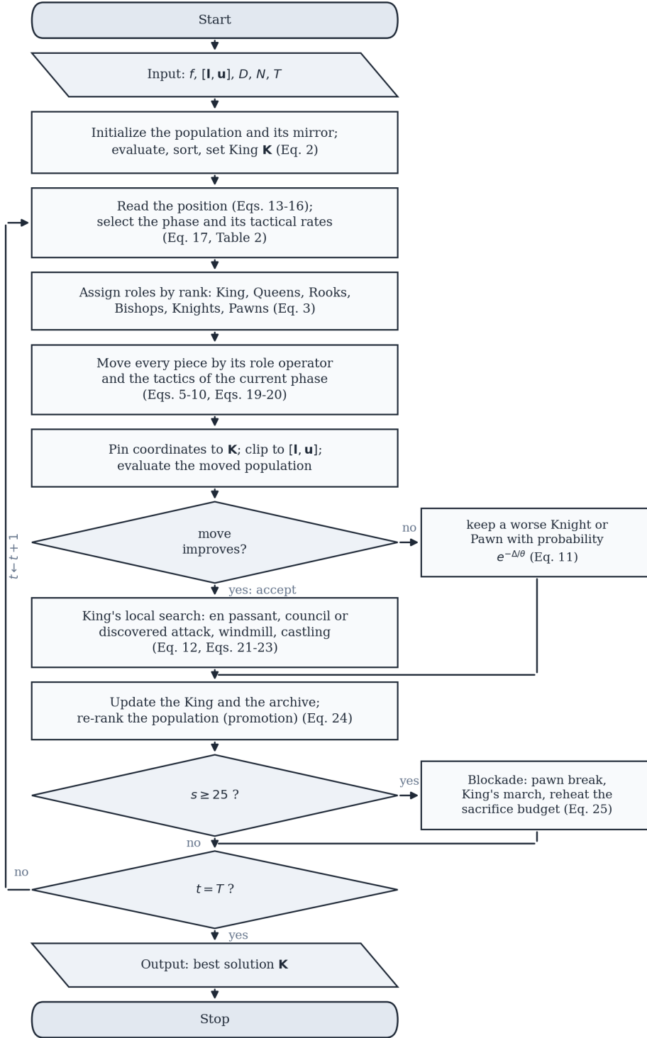
Figure 3: Flowchart of the Chess Algorithm.
