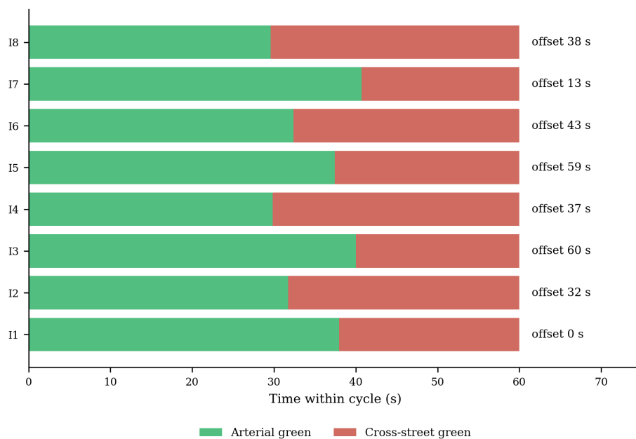
Figure 20: Time-space representation of the best plan found by CA.
