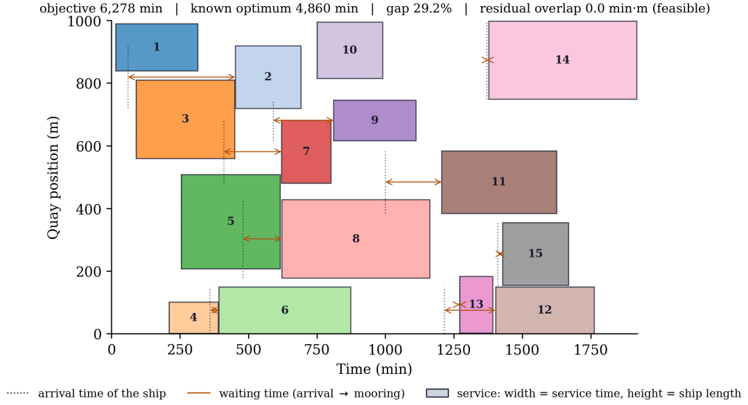
Figure 22: Best berth allocation plan found by CA. One rectangle per ship, no overlap, so the plan is feasible; the gap to F^* is waiting time alone.
