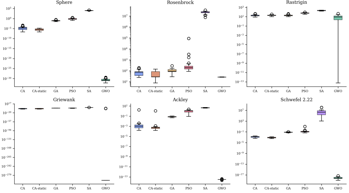
Figure 8: Distribution of final objective values over 30 runs.
