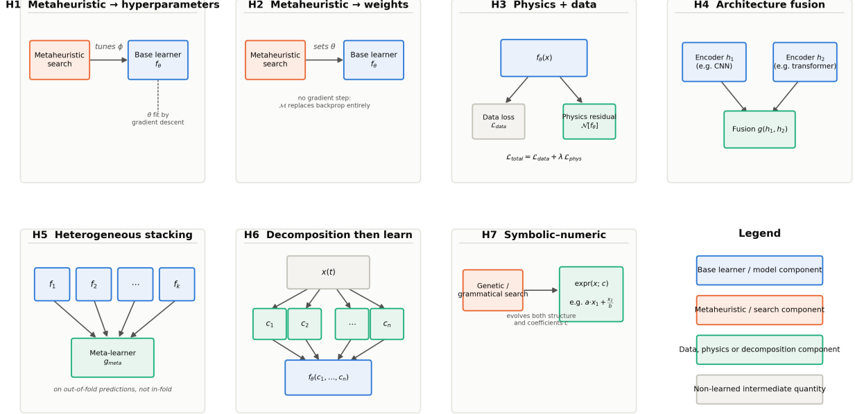
Figure 6: Schematic architecture of the seven hybridisation types. Boxes shown in the same colour play the same structural role across panels (base learner, search component, or data/physics/decomposition component); the diagram sets out the general coupling each type names, not any one paper's specific implementation.
