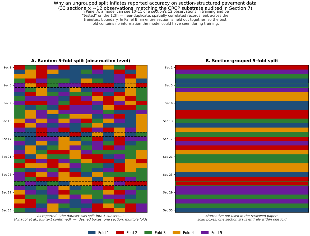
Figure 4: Random versus section-grouped 5-fold cross-validation on a 33-section, ~12-observation-per-section substrate matching the CRCP data audited in this section. Panel A reproduces the partitioning [22]’s methods section describes; Panel B shows the section-grouped alternative not used in the reviewed papers.
