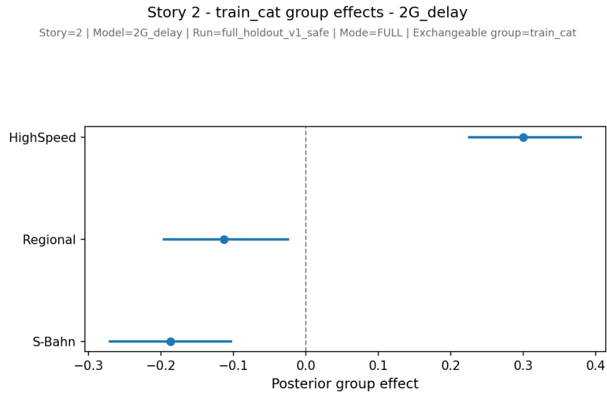
Figure 45: train_cat effects for Story 2 grouped Binomial.
