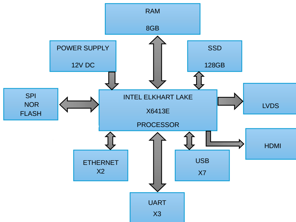
Figure 1: Block Diagram of Single Board Computer (SBC)
