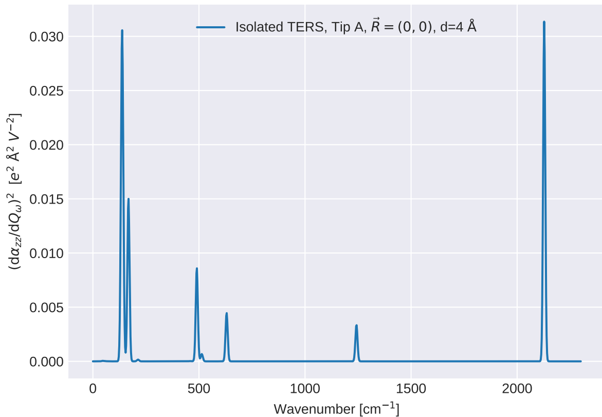
TCNE harmonic zz-Raman, Gaussian-broadened by \sigma = 5 \text{ cm}^{-1}
