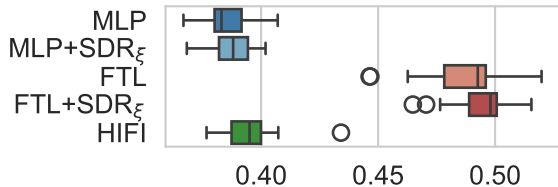
Statistical Parity
