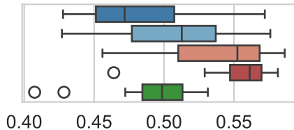
Equal Opportunity
