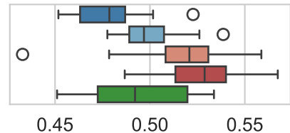
Equalized Odds
