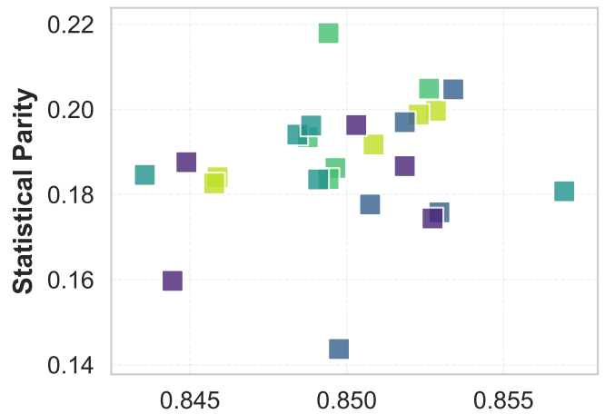
MLP+SDR ξ
