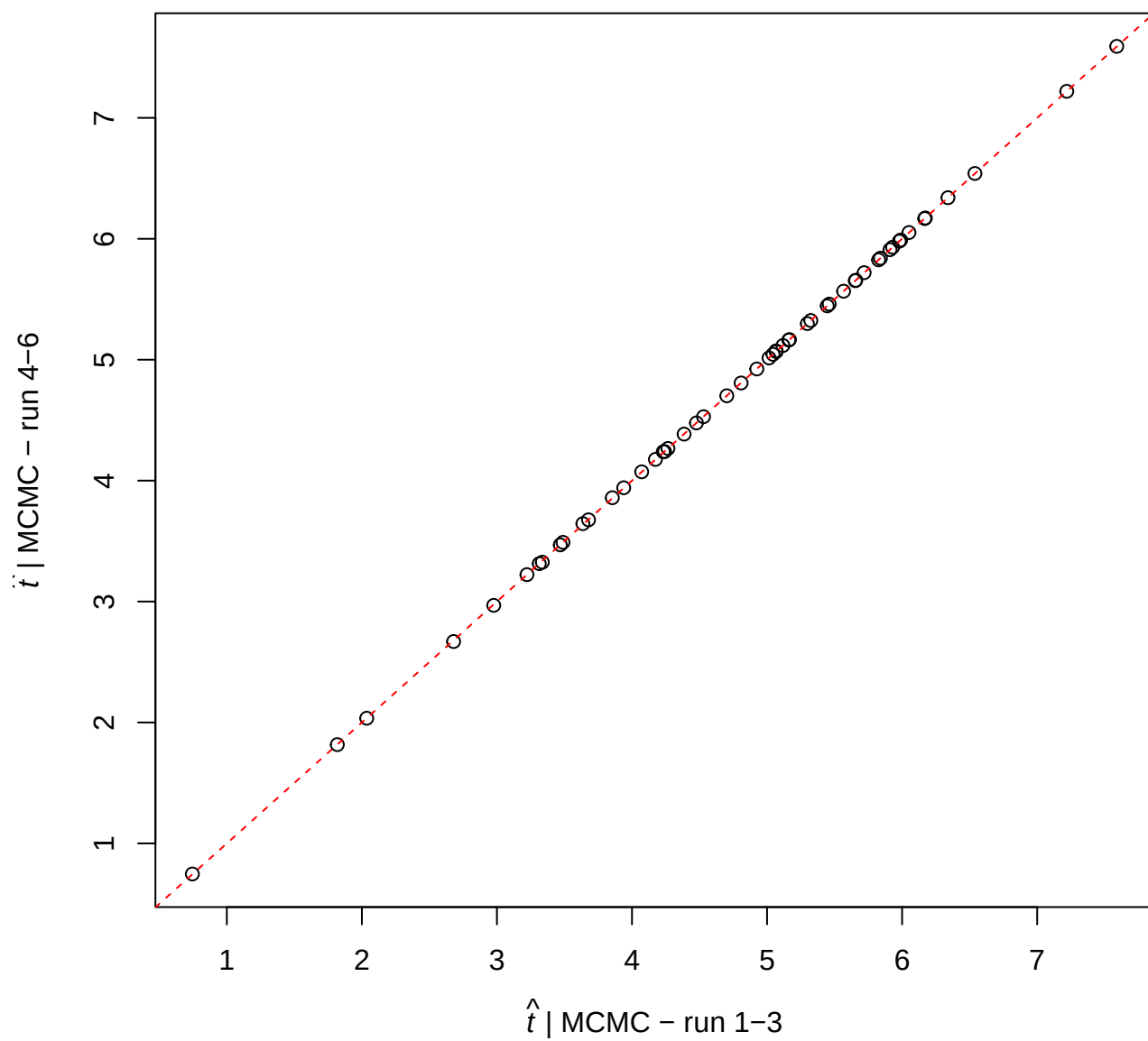
Convergence plot – post_Unconstrained-ILN
