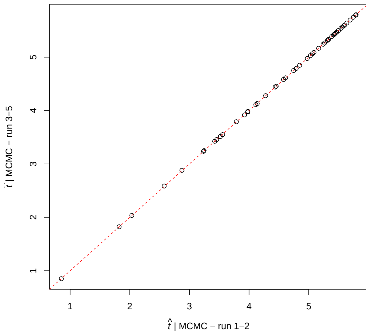
Convergence plot – post_UpperEdiacaran–ILN (FILT)
