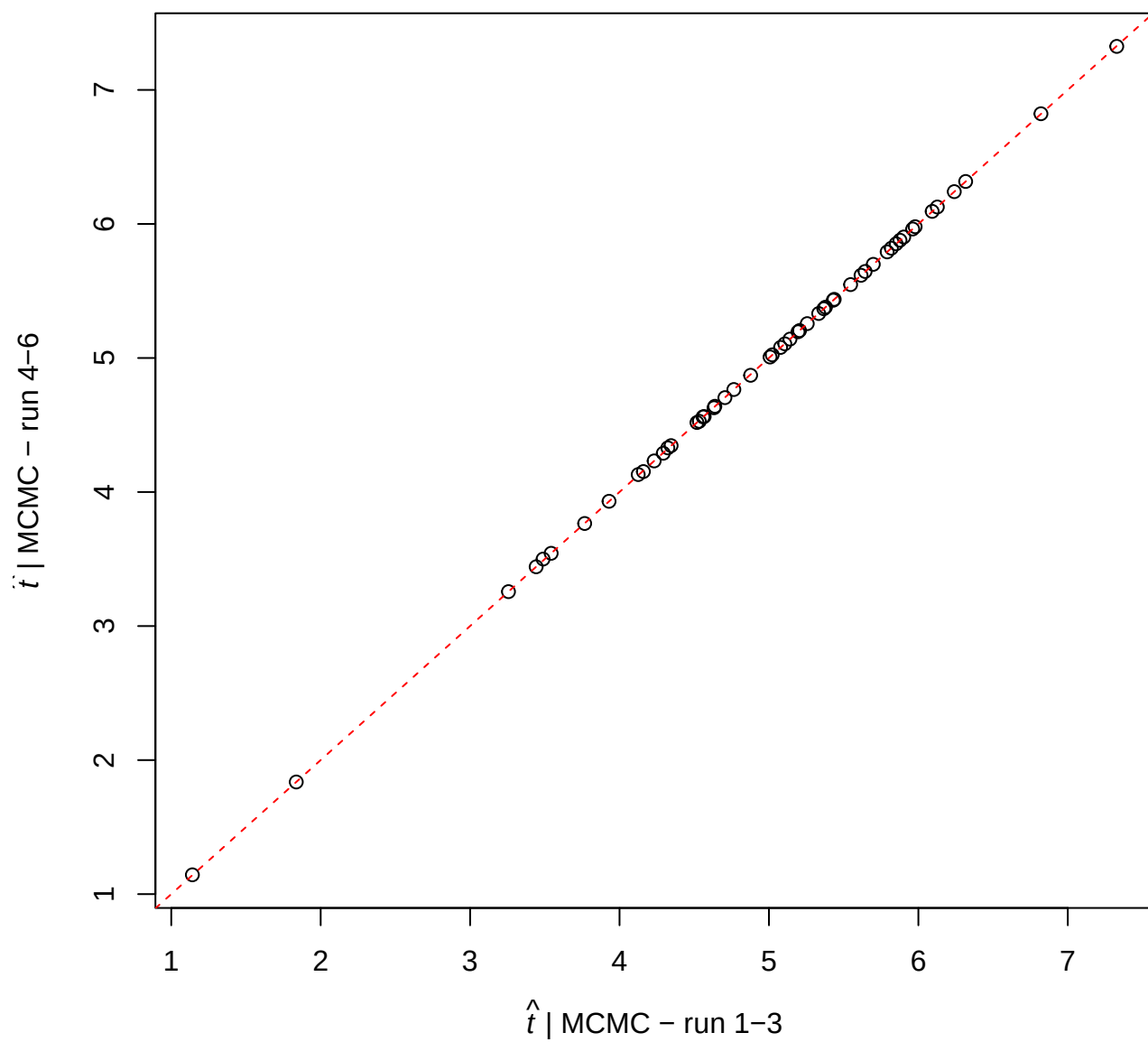
Convergence plot – prior_Unconstrained–NODAT–ILN
