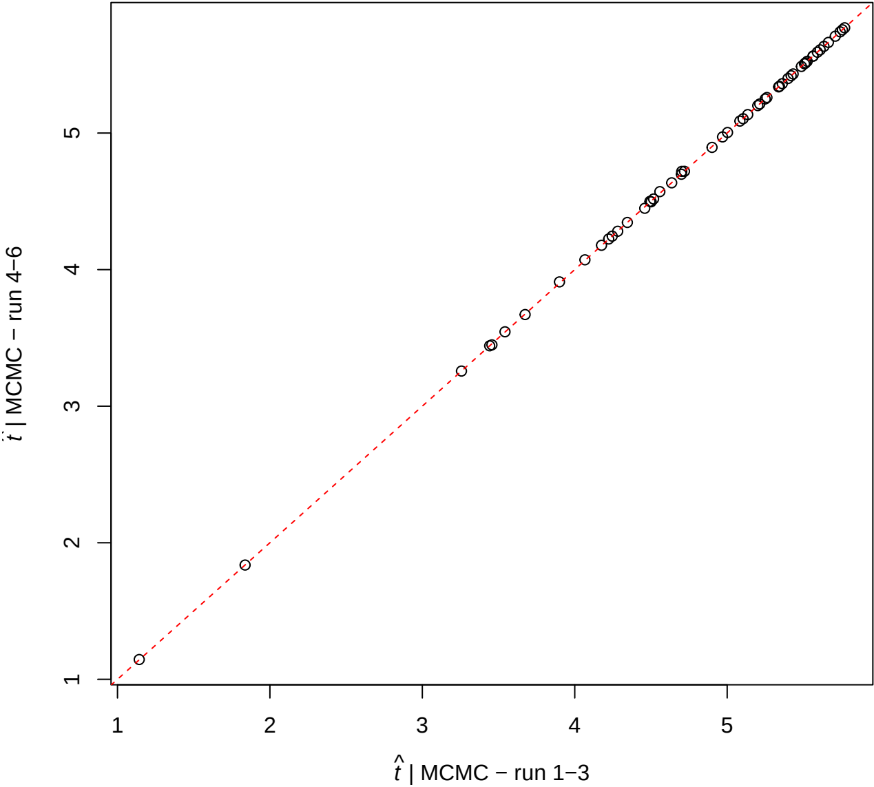
Convergence plot – prior_UpperEdiacaran–NODAT–ILN
