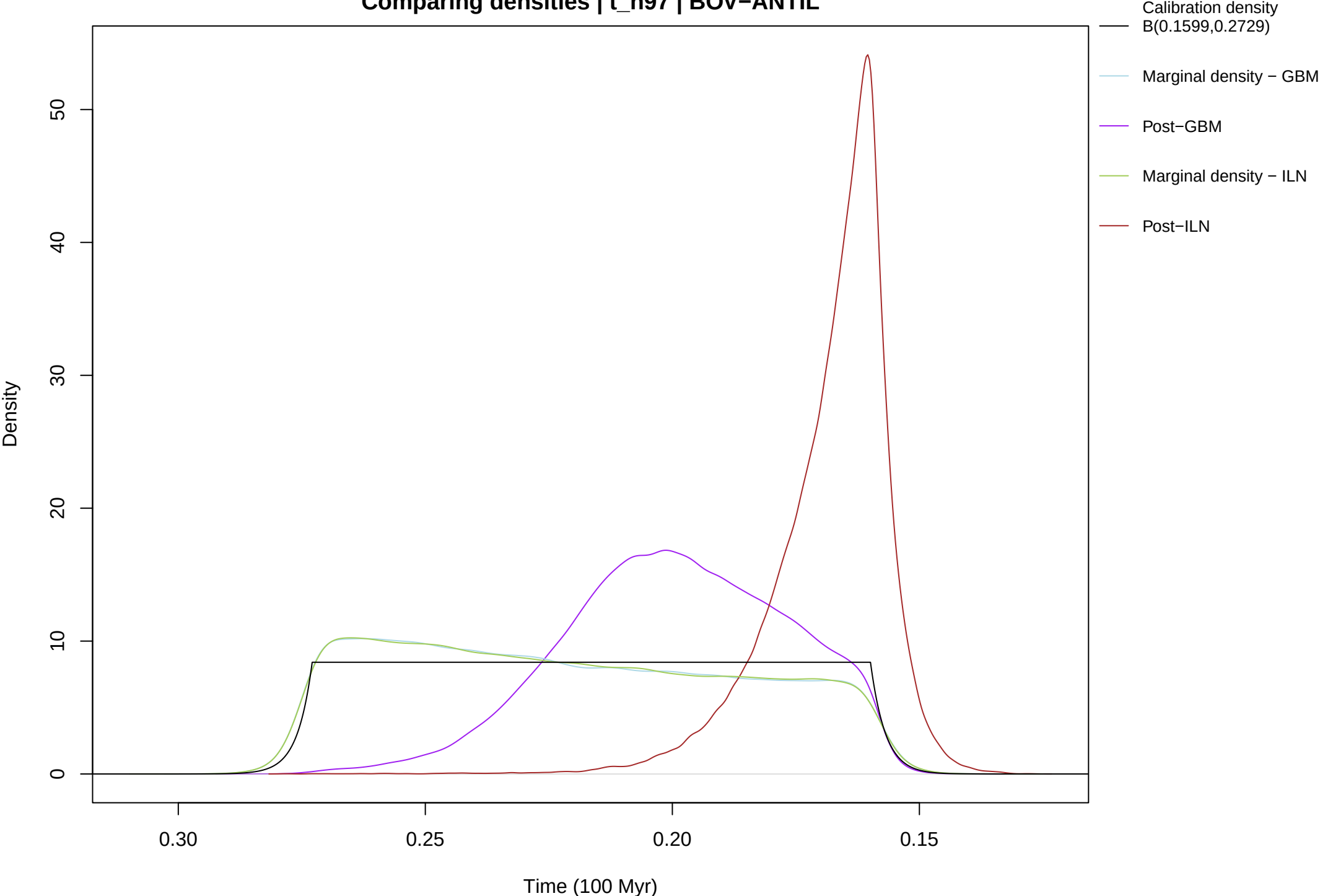
Comparing densities | t_n97 | BOV-ANTIL
