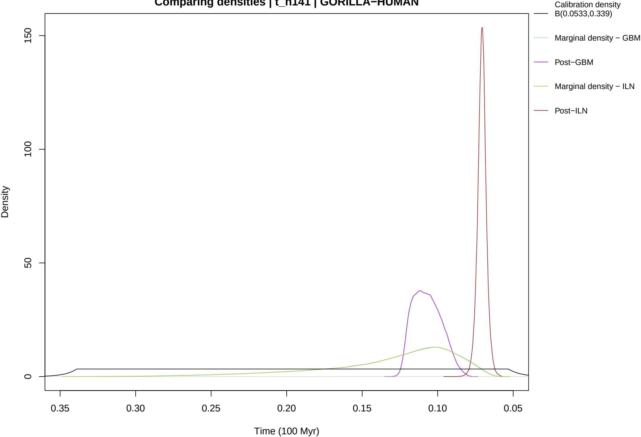
Comparing densities | t_n141 | GORILLA-HUMAN
