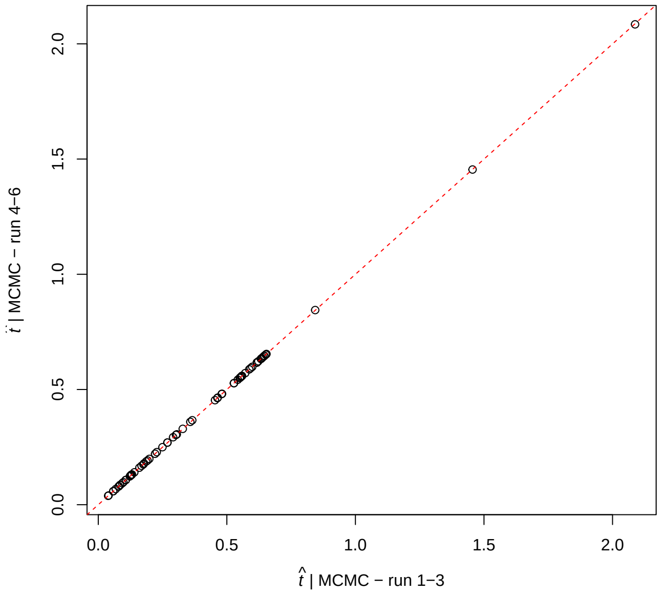
Convergence plot – prior_PostKPg–NODAT–ILN
