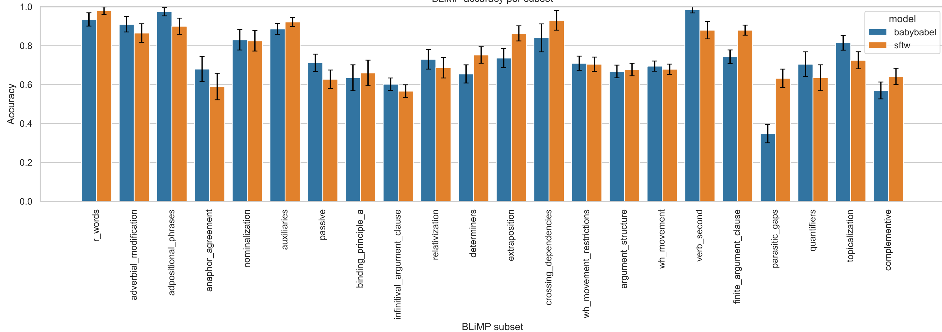
BLiMP accuracy per subset
