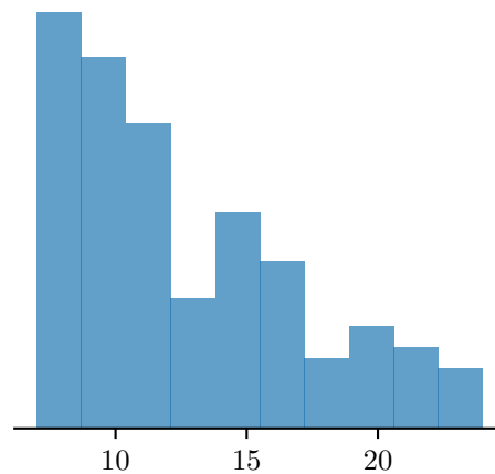
Subset = 0.9
