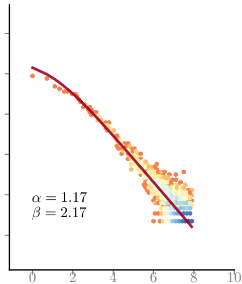
Subset: 0.9
