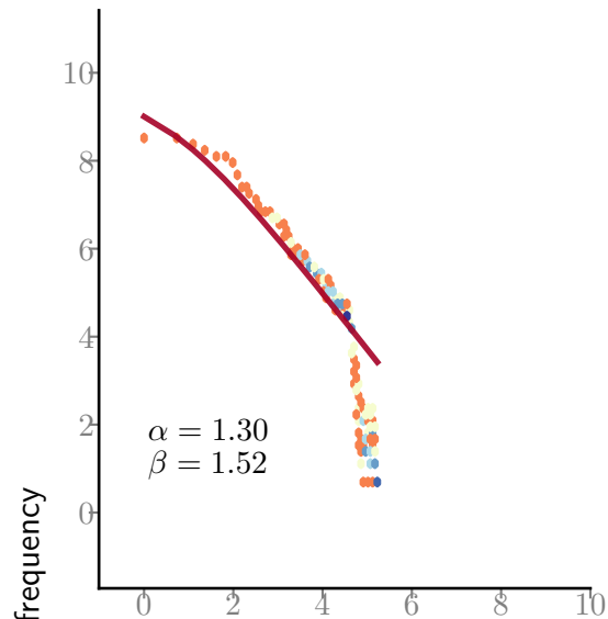
Subset: 0.6
