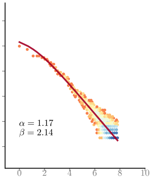
Subset: 0.8
