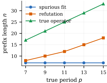
(a) planted deception D_j
