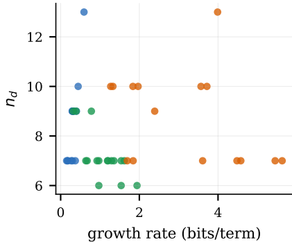
(b) growth is irrelevant ( r = -0.007 )
