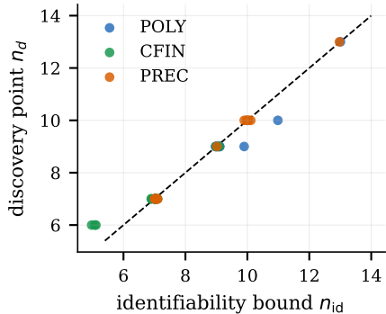
(a) n_d = n_{id} : 89% exact
