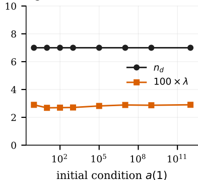
(c) growth invariance (Fibonacci)
