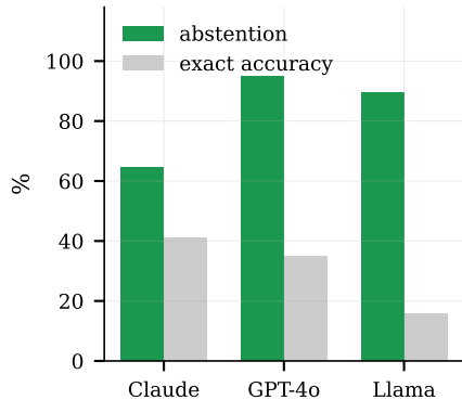
(c) models hedge in the wilderness
