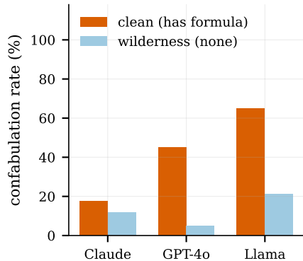
(a) confident errors are inverted
