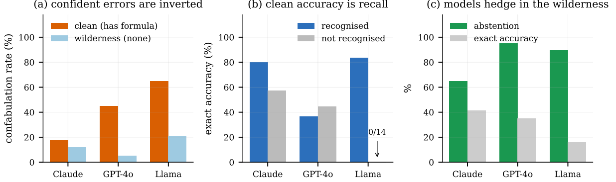
Figure 5: Language-model behaviour by MDL stratum. (a) Confabulation rate— stated confidence \geq 4 with a wrong continuation— on the clean stratum (orange) against the wilderness (light blue): confident errors concentrate on the easy stratum, not the hard one. (b) Clean-stratum exact accuracy split by whether the model reported recognising the sequence (blue) or not (grey); Llama scores 0/14 without recognition. (c) In the wilderness, abstention (green) against exact accuracy on the next three terms (grey): all three models hedge, refuting our pre-registered hypothesis. All three panels are percentages on a fixed 0–100 scale.
