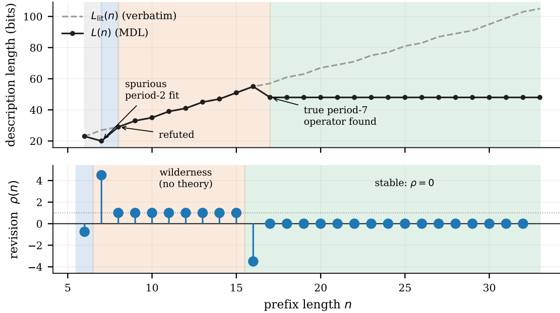
Figure 2: The five phases of a revision spectrum on the planted deceptive sequence D_3 (true period 7). Top: MDL codelength L(n) against the verbatim cost L_{lit}(n) , shaded by the phase holding at n —literal (grey), spurious period-2 fit (blue), wilderness (orange), stable (green). Bottom: the normalized revision \rho(n) . Since \rho(n) is indexed by its source prefix length, the revision at n is what installs the state at n+1 ; the shading in the lower panel is shifted one step left accordingly, so each spike is coloured by the phase it leads into.
