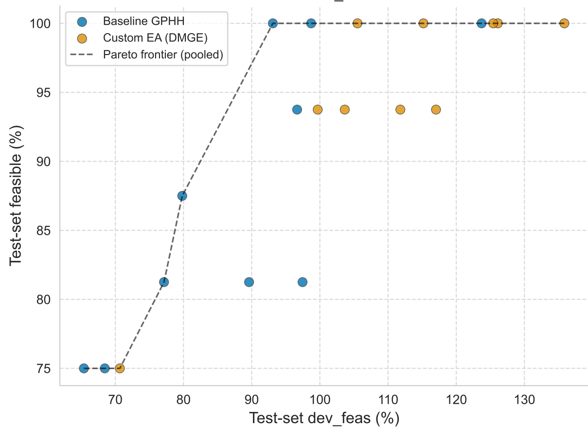
PSPLIB_J20
