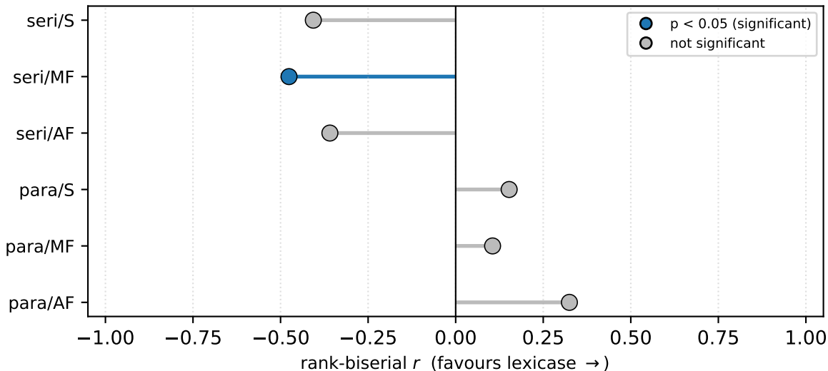
Lexicase vs. baseline: effect size per cell (MMLIB50)
