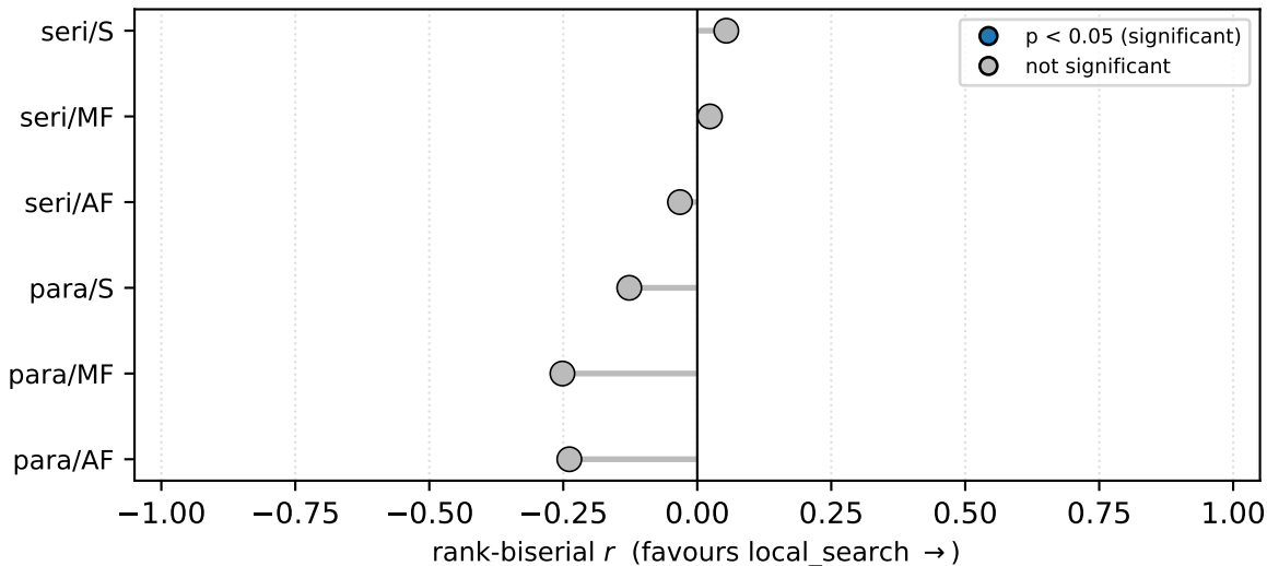
Local search vs. baseline: effect size per cell (MMLIB100)
