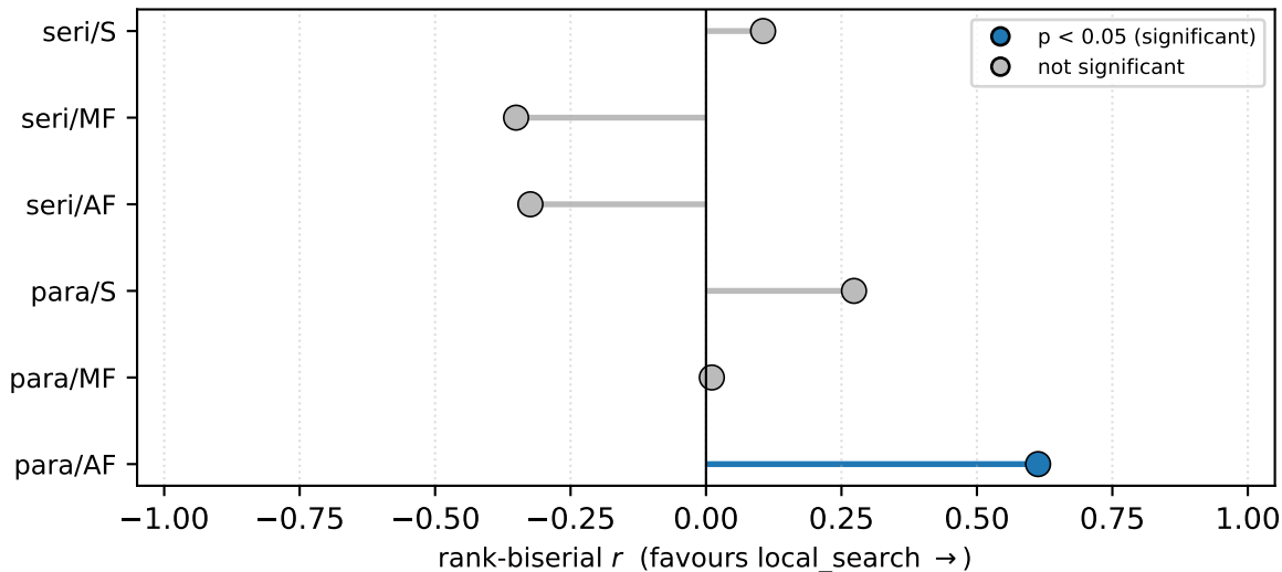
Local search vs. baseline: effect size per cell (MMLIB50)
