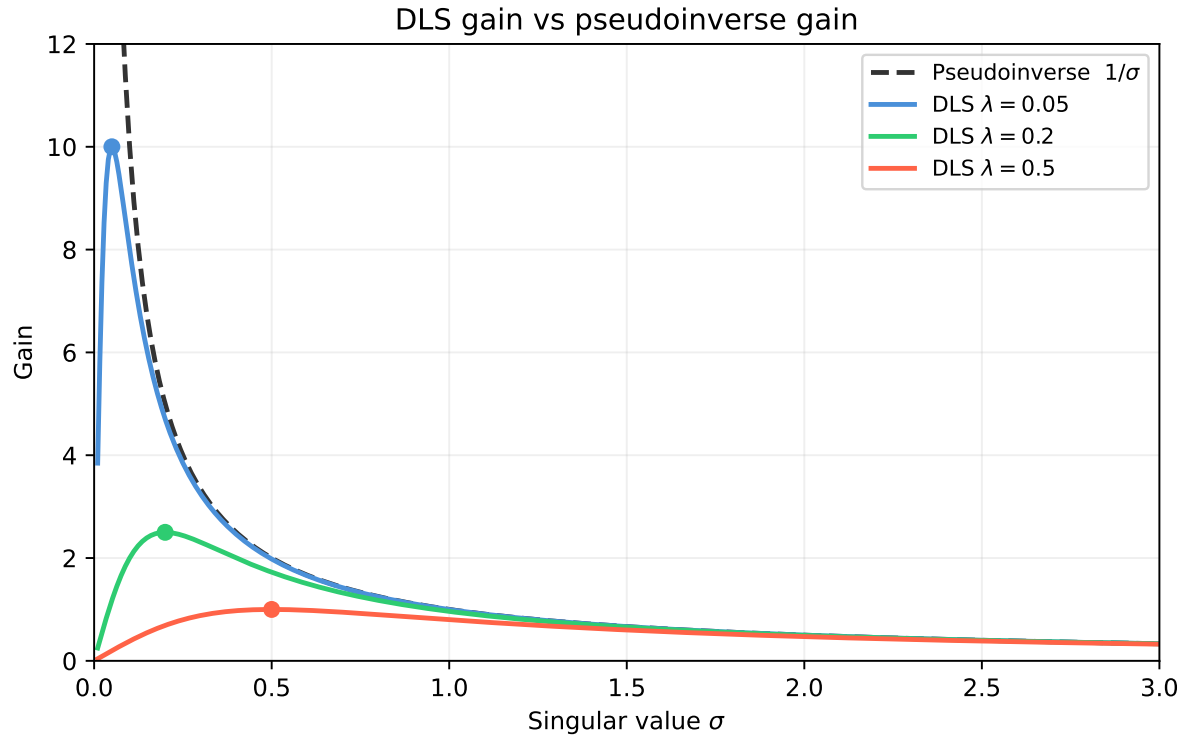
Figure 22.6.: Gain as a function of singular value \sigma for the pseudoinverse ( 1/\sigma ) and DLS ( \sigma/(\sigma^2 + \lambda^2) ) at three damping levels. DLS stays bounded near \sigma=0 .
