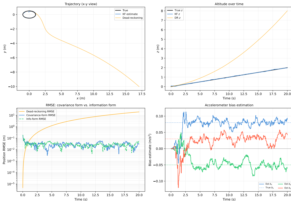
Figure 23.7.: Simulated RealSense + IMU fusion. Top: true trajectory (black) vs. dead-reckoning on IMU alone (orange) vs. EKF fused estimate (blue). Bottom-left: position RMSE over time. Bottom-right: accelerometer bias estimate converging to the true injected bias.
