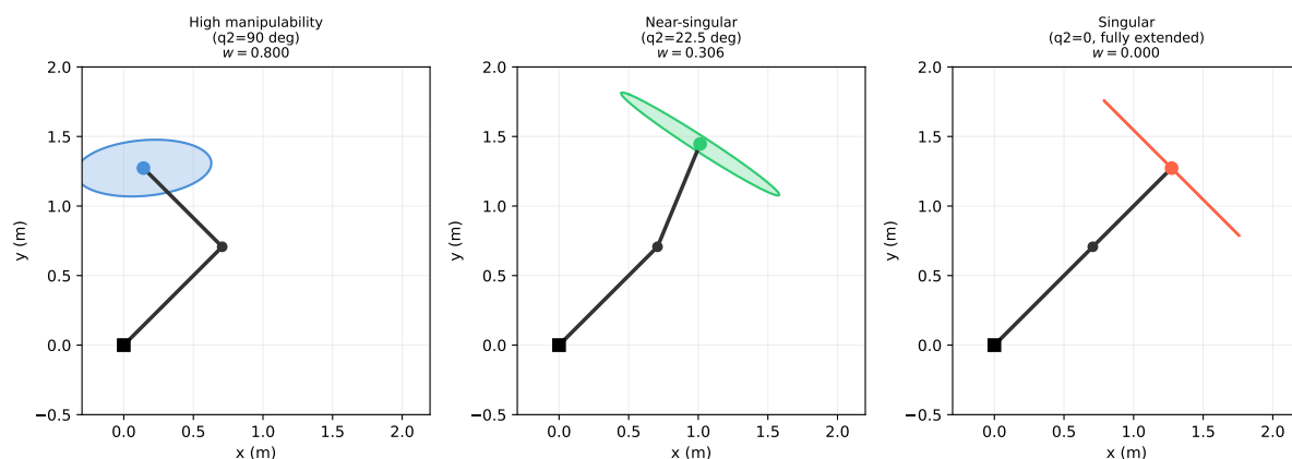
Figure 22.4.: Three arm configurations: high manipulability (left), near-singular (center), and singular (right, q_2=0 — arm fully extended).
