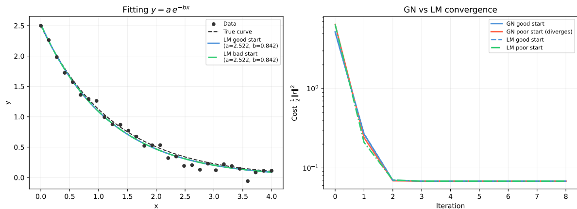
Figure 22.8.: LM vs Gauss-Newton on a nonlinear least-squares problem: fitting y = a * \exp(-b*x) to noisy data. LM converges reliably from a poor initial guess; GN diverges.
