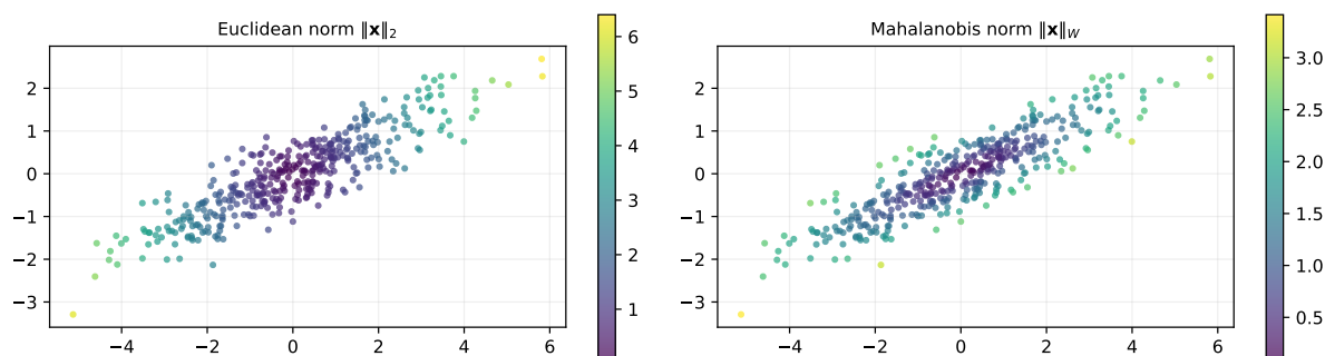
Same data, different inner product -- different sense of distance
