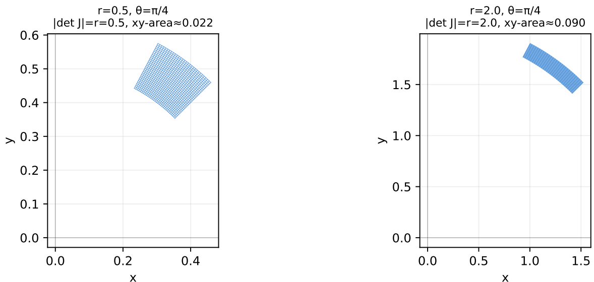
Polar map: small rectangle in (r, \theta) maps to a curved patch
