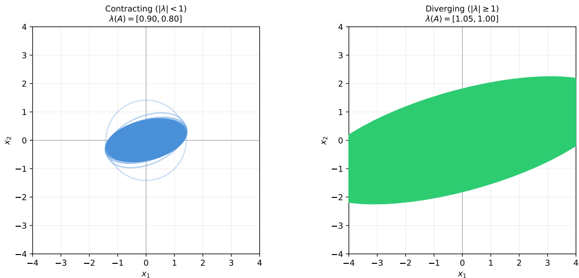
Figure 23.2.: Covariance ellipse propagation for a 2D system (no measurements). Left: contracting dynamics. Right: diverging dynamics. Ellipses are drawn every 3 steps; the final ellipse is filled.
