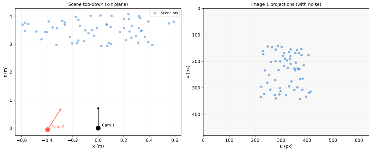
Figure 25.7.: Synthetic 3D scene: 60 random scene points and two cameras. Left: top-down view (x-z plane) showing camera positions and optical axes. Right: image 1 projections.
