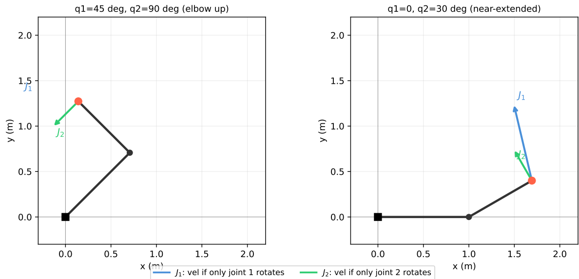
Figure 22.2.: Jacobian columns as end-effector velocity arrows. Blue arrow: velocity when only joint 1 rotates. Green arrow: velocity when only joint 2 rotates.
