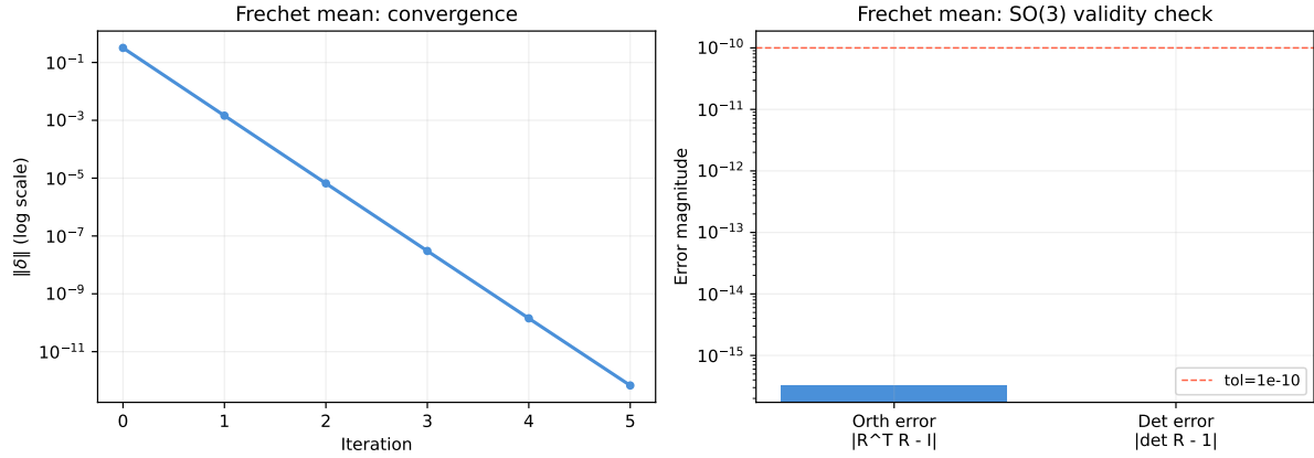
Figure 24.7.: Riemannian gradient descent for rotation averaging. The algorithm converges in fewer than 20 iterations even with 20 rotations spread over a 60-degree ball.
