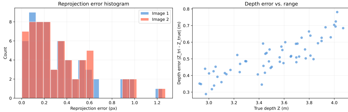
Figure 25.9.: Reconstruction quality: reprojection error for all 60 points using the estimated F and recovered pose. Mean reprojection error is typically under 1 pixel at 0.5 px noise.
