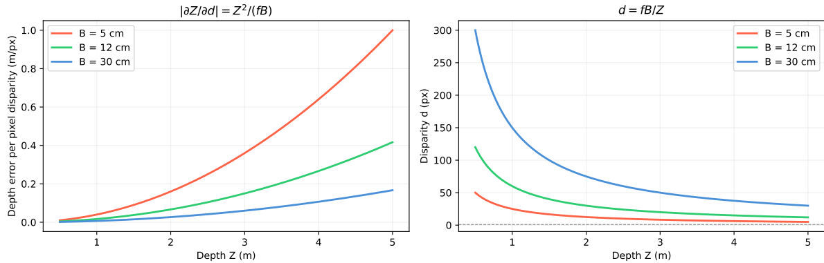
Figure 25.6.: Stereo depth precision as a function of range for three baselines ( f = 500 px). Depth precision degrades as Z^2 , and wider baselines (blue > green > orange) recover precision.
