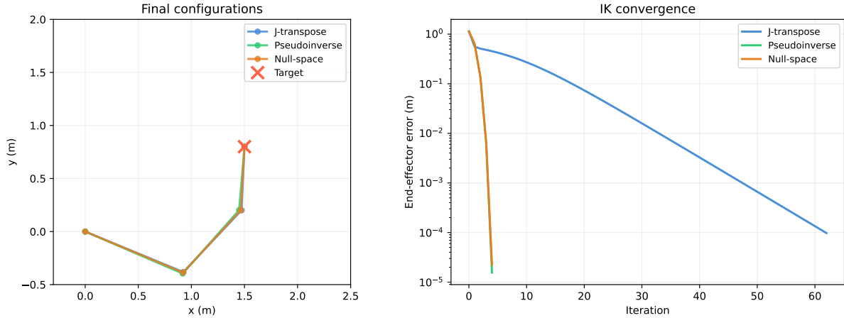
Figure 22.5.: IK trajectories for a 3-link planar arm: Jacobian-transpose (blue), pseudoinverse (green), and pseudoinverse + null-space manipulability gradient (orange). All reach the target (red cross) from the same start.
