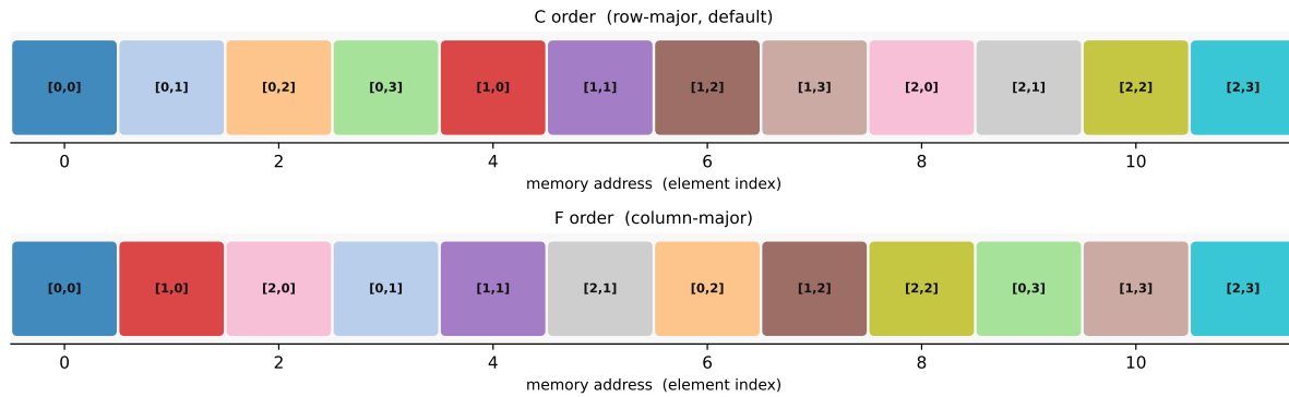
Figure 26.1.: A 3x4 matrix stored in memory under C order (row-major, top) and F order (column-major, bottom). Each cell shows the matrix position [row,col]; its horizontal position is its slot in the flat memory buffer.
