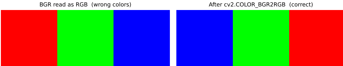
Figure 26.2.: A synthetic test image displayed without and with BGR-to-RGB conversion. OpenCV’s pure-blue patch [255, 0, 0] in BGR appears red when matplotlib reads it as RGB (left). After cv2.cvtColor(img, cv2.COLOR_BGR2RGB) the colors are correct (right).
