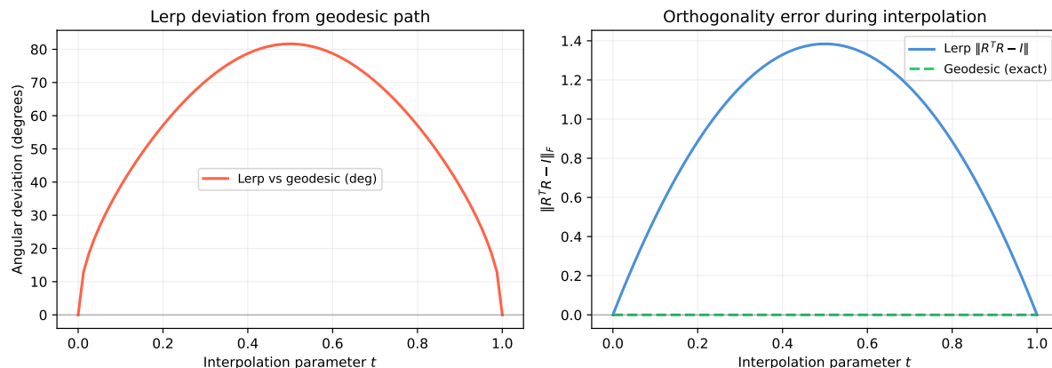
Figure 24.5.: Geodesic interpolation on SO(3) vs naive matrix lerp. Left: angular separation between interpolated frame and the exact geodesic. Right: orthogonality error \|R^T R - I\|_F . Geodesic stays on SO(3) ; lerp drifts off.
