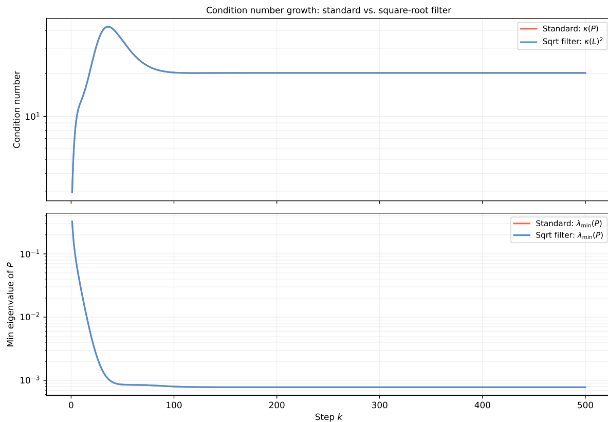
Figure 23.5.: Numerical stability of standard vs. square-root Kalman filter over 500 steps. Top: condition number of P (standard) vs. \text{cond}(L)^2 (square-root). Bottom: smallest eigenvalue of P ; the standard form eventually produces near-zero or slightly negative eigenvalues while the square-root form maintains strict positivity.
