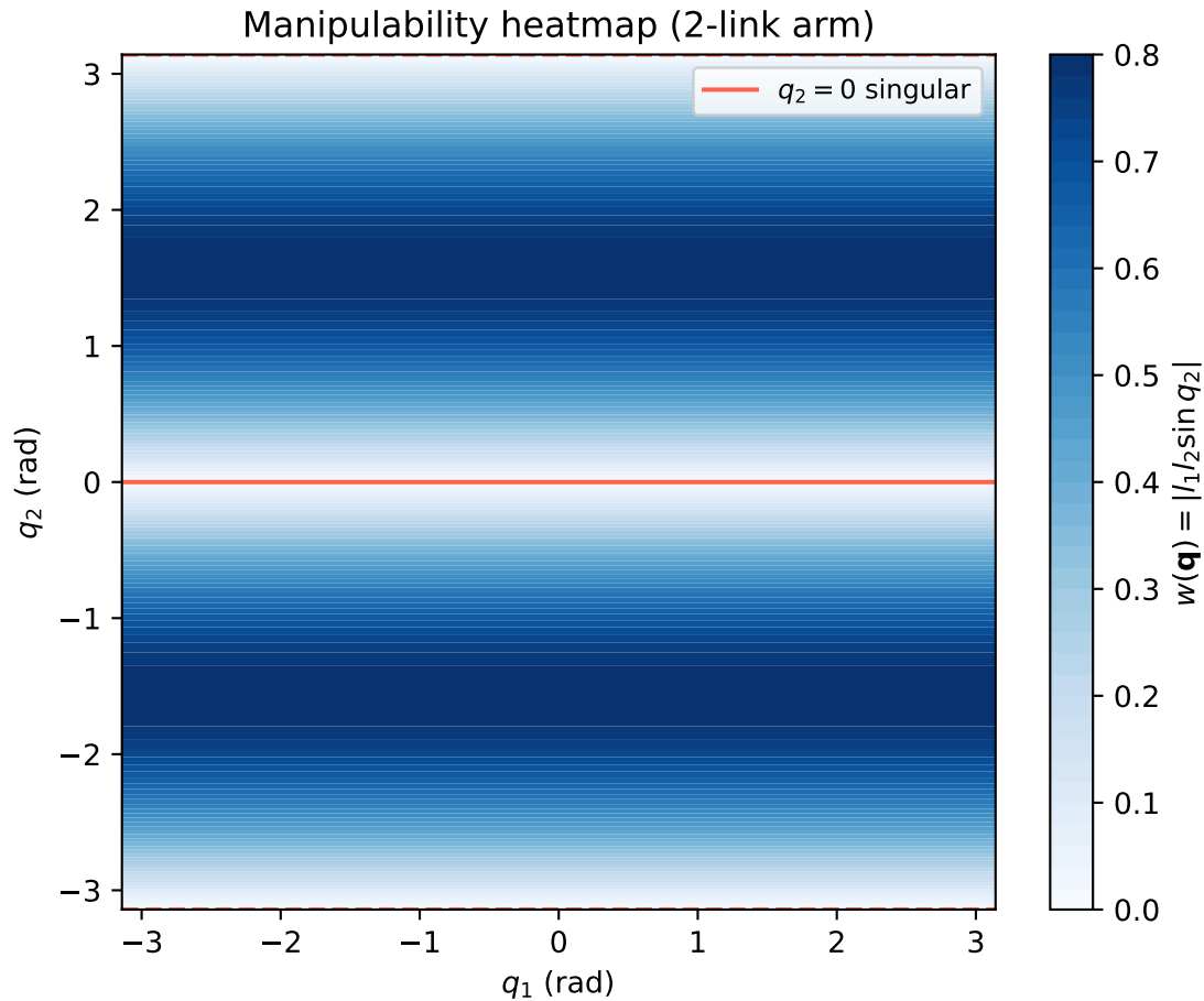
Figure 22.3.: Manipulability w(\mathbf{q}) = |l_1 l_2 \sin(q_2)| for the 2-link arm. Singularities ( w=0 ) occur at q_2=0 and q_2=\pi (white bands).
