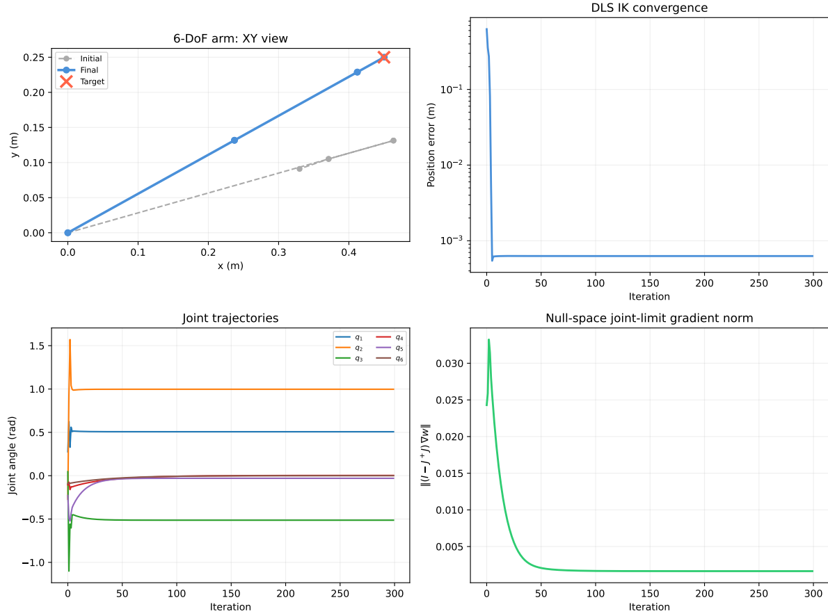
Figure 22.9.: DLS IK for a 6-DoF arm (simplified Puma-style DH parameters). Top left: FK arm at final configuration. Top right: IK convergence. Bottom: joint angles over iterations and null-space joint-limit gradient norm.
