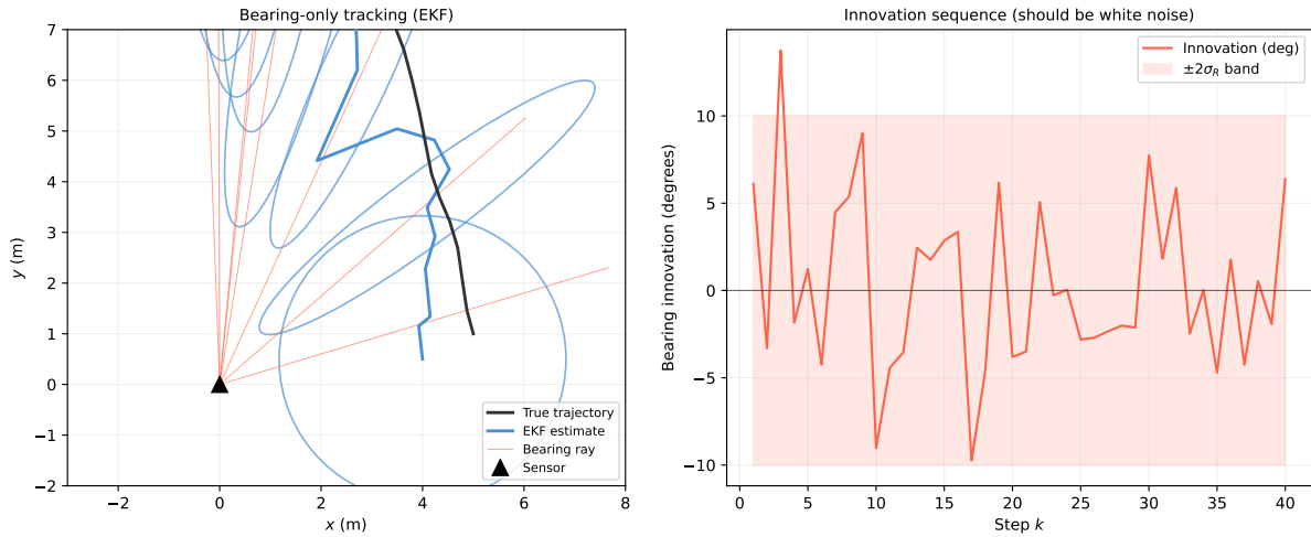
Figure 23.6.: EKF bearing-only tracking. Left: true trajectory (black), noisy bearing measurements projected as rays (red), EKF position estimate (blue) with 2-sigma covariance ellipses every 5 steps. Right: bearing innovation sequence, which should be zero-mean white noise for a well-tuned filter.
