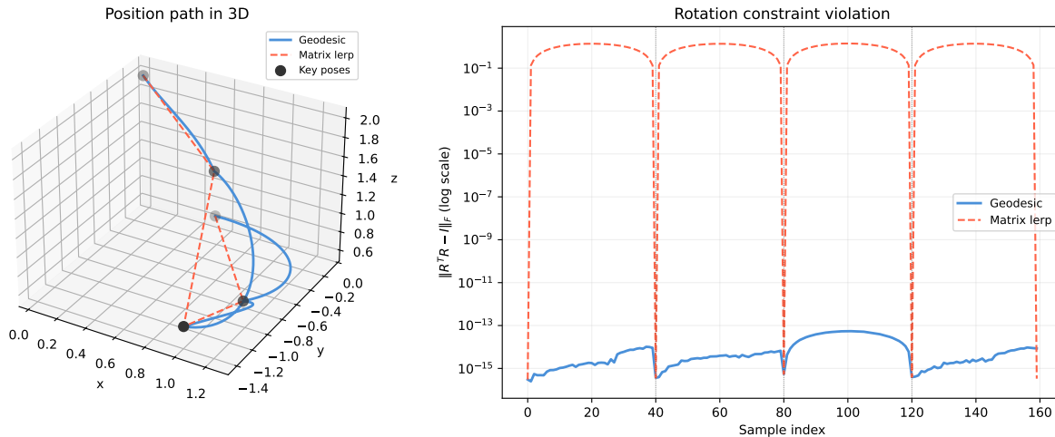
Figure 24.9.: 6-DoF geodesic trajectory (blue) vs naive matrix-lerp (orange) through 5 key poses. Left: position path in 3D. Right: orthogonality error of the rotation block – geodesic stays at machine precision; lerp drifts.
