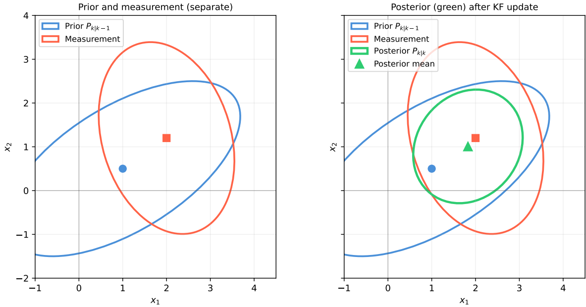
Figure 23.3.: Kalman update as an ellipse merge. Left: prior (blue) and measurement likelihood (red). Right: posterior (green) lies inside both ellipses, closest to whichever is tighter.
