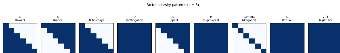
Figure 27.1.: Sparsity patterns of the factor matrices produced by each decomposition for a 6x6 example. Dark cells are non-zero entries; light cells are structural zeros. L (lower triangular), U (upper triangular), Q (orthogonal – dense), R (upper triangular), P (eigenvector matrix – dense), and U/V T (singular vector matrices – dense).
