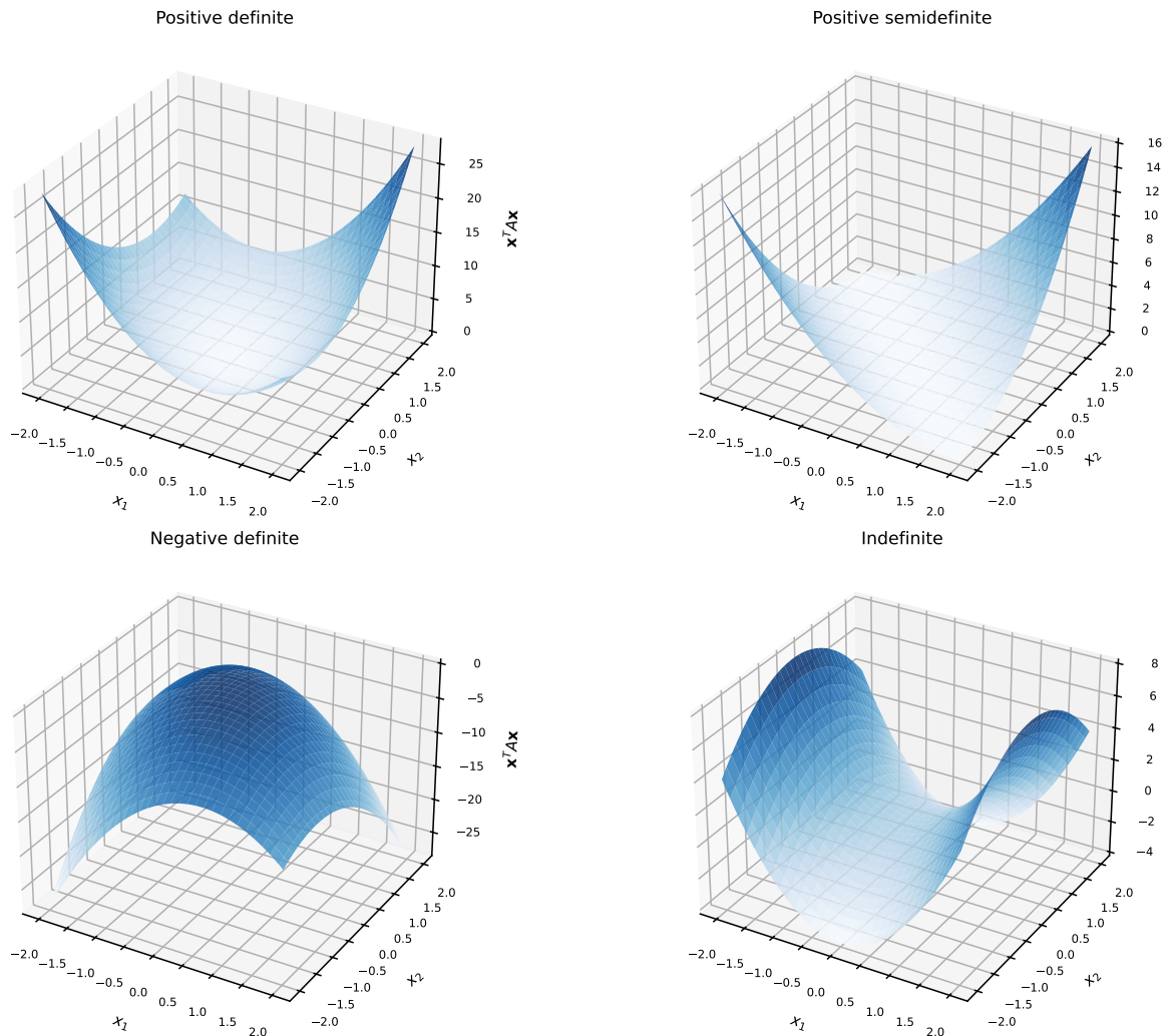
Quadratic form \mathbf{x}^T \mathbf{A} \mathbf{x} for four definiteness types
