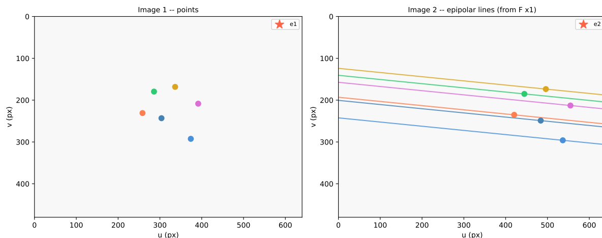
Figure 25.3.: Epipolar lines generated by the fundamental matrix. Six color-coded points in image 1 (left) each generate a corresponding epipolar line in image 2 (right). The match for each point must lie on its colored line.
