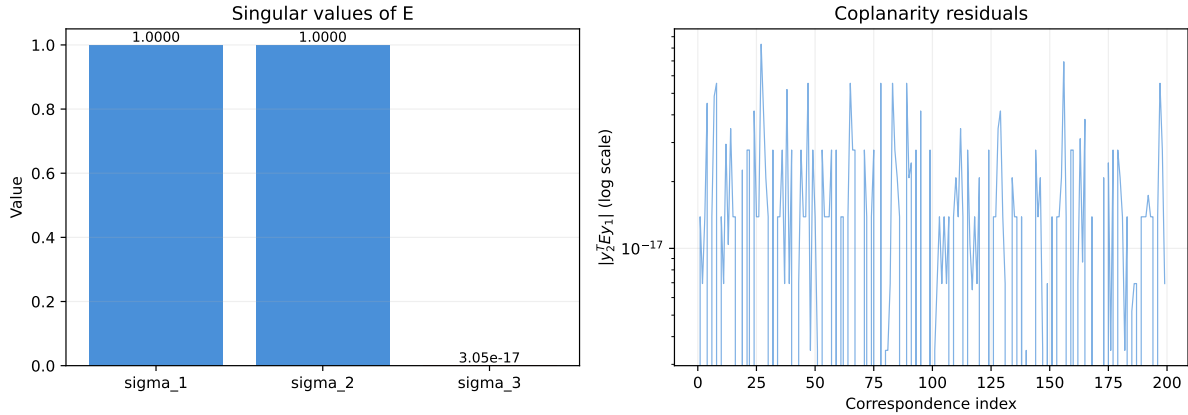
Figure 25.2.: Singular values of E and the algebraic residual |\mathbf{y}_2^T E \mathbf{y}_1| for 200 random calibrated correspondences. Left: the two nonzero singular values are exactly equal by construction. Right: residuals are at machine-precision zero, confirming the coplanarity constraint.
